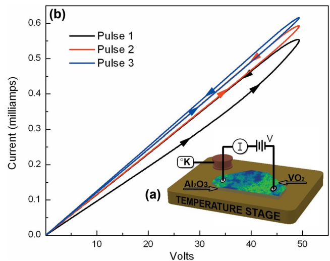
FIG. 1. (Color online) (a) Schematic of the device. The area of the VO 2 film is ~25 mm 2 . (b) Three current-voltage ( I-V ) curves for our device exhibiting nonlinear hysteretic behavior which is indicative of a memristive system.
