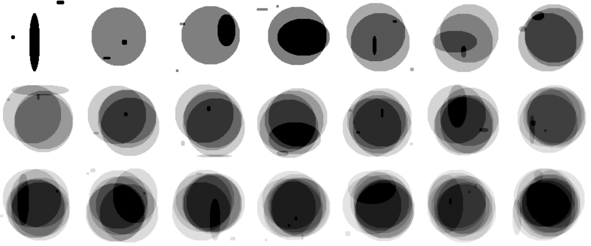
Figure 9. Random images with varying cosparsity \ell = p - k , parametrized by \rho (6.2). For each dimension d = 80 \dots 180 , random images were generated for \rho = 0.005 \dots 0.22 . The figure shows a sample image for a subset of increasing values of \rho and d = 120 .
