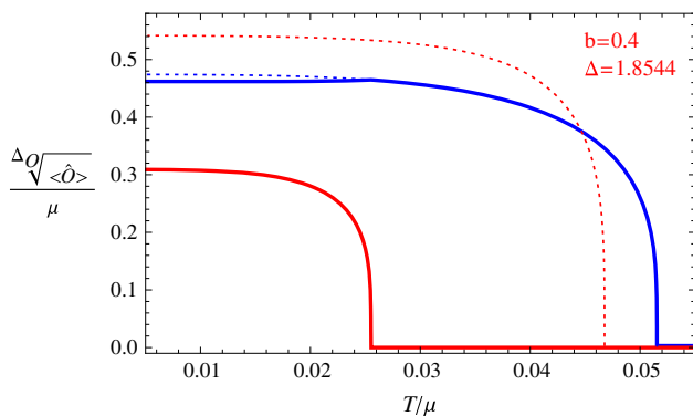
Fig. 3 The condensation of the s-wave and p-wave orders. The red line denotes the value for the p-wave order, and the blue line denotes the value for the s-wave order. Dotted lines are for unstable phases and solid lines for stable phases
