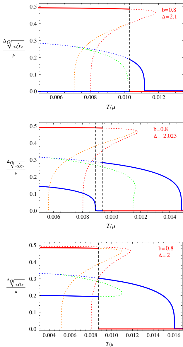
Fig. 5 The condensation value of the s-wave and p-wave orders. The red line denotes the value for the p-wave order, and the blue line denotes the value for the s-wave order. Dotted lines are for unstable phases and solid lines for stable phases. The dotted orange line and dotted green line denote the condensation value for the p-wave and s-wave orders in the unstable part of the s + p solution. We use the vertical dashed black lines to mark the critical temperatures between the condensed phases clearly
