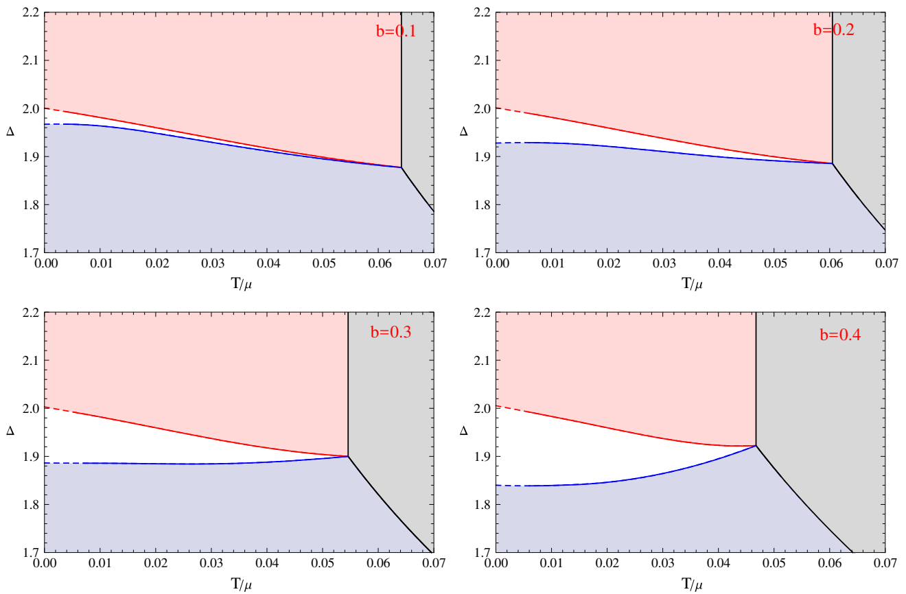
Fig. 7 The \Delta - T phase diagrams for b values from 0.1 to 0.4. In these figures, the areas colored by light gray, light blue, light red and white denote the normal phase, the s-wave phase, the p-wave phase and the s + p coexisting phase respectively. The black curves are made up by phase transition critical points between the s-wave or p-wave phases and the normal phase. The solid red curves describe the second order phase
