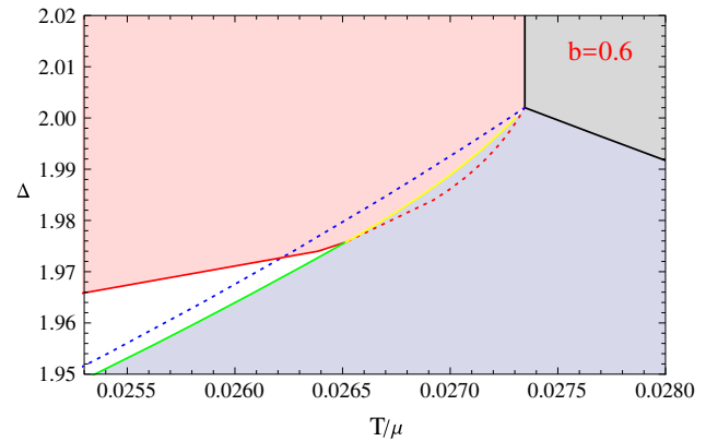
Fig. 9 The enlarged version of the \Delta - T phase diagrams for the case with b = 0.6
