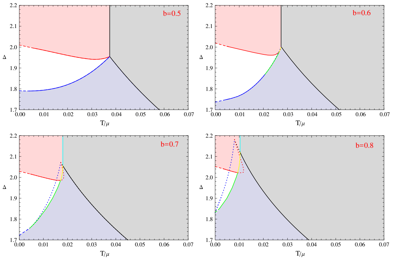
Fig. 8 The \Delta - T phase diagrams for b values from 0.5 to 0.8. In these figures, the solid cyan line denotes the critical points of the first order phase transitions from the normal phase to the p-wave phase. The solid yellow lines represent the first order phase transition critical points from s-wave phases to p-wave phases. The solid green lines represents the
