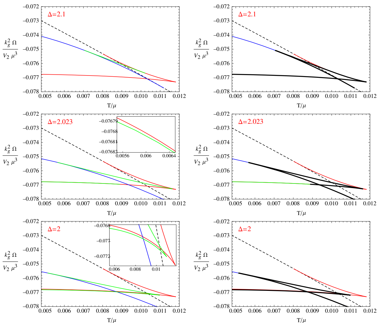
Fig. 6 The free energy of the different phases with b = 0.8 . The first two figures are for the case \Delta = 2.1 , the third and fourth figures are for the case \Delta = 2.023 and the fifth and sixth ones for \Delta = 2 . In the three figures on the left side, the dashed black line denotes the free energy for the normal phase, the solid red line and solid blue line denotes the free energy of the p-wave phase and s-wave phase respectively, the solid
