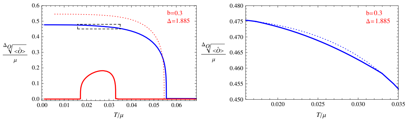
Fig. 2 The condensation value of the s-wave and p-wave orders. The red line denotes the value for the p-wave order, and the blue line denotes the value for the s-wave order. Dotted lines are for unstable phases and
