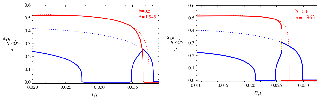
Fig. 4 The condensation value of the s-wave and p-wave orders. The red line denotes the value for the p-wave order, and the blue line denotes the value for the s-wave order. Dotted lines are for unstable phases and
