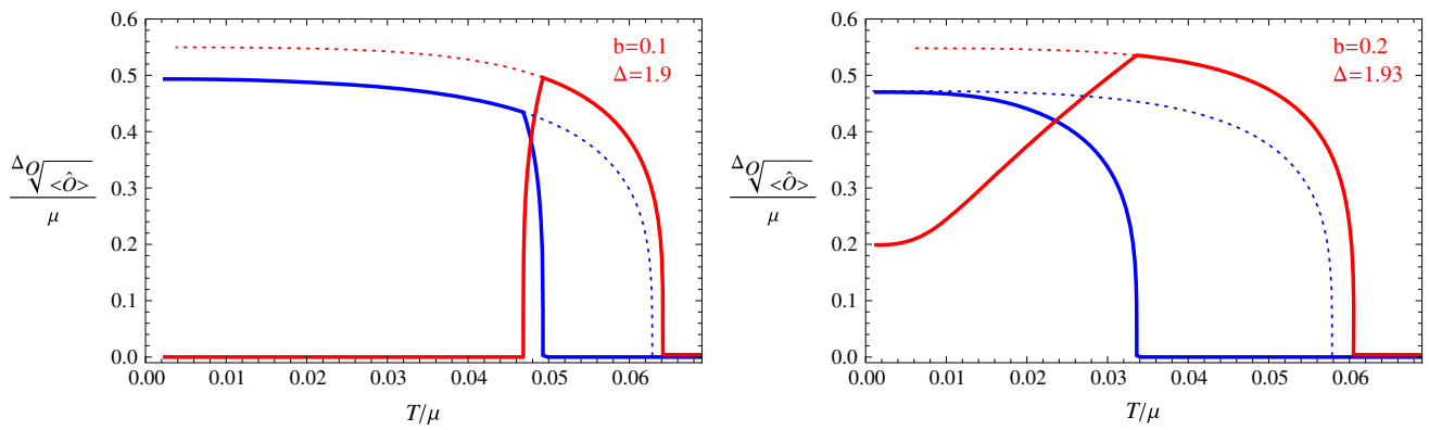
Fig. 1 The condensation value of the s-wave and p-wave orders. The red line denotes the value for the p-wave order, and the blue line denotes the value for the s-wave order. Dotted lines are for unstable phases and solid lines for stable phases
