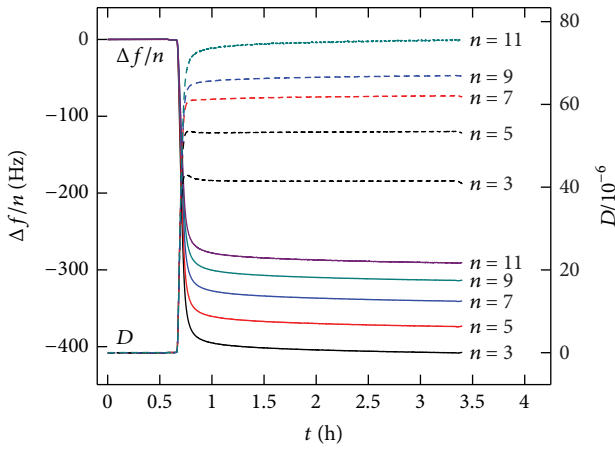
FIGURE 8: Time evolution of \Delta f/n (solid lines) and \Delta D (dashed lines) during a typical QCM-D experiment of vesicle adsorption on gold-coated quartz at 16^\circ\text{C} . Data for the DMPC + 0.1 DSPC mixture.
