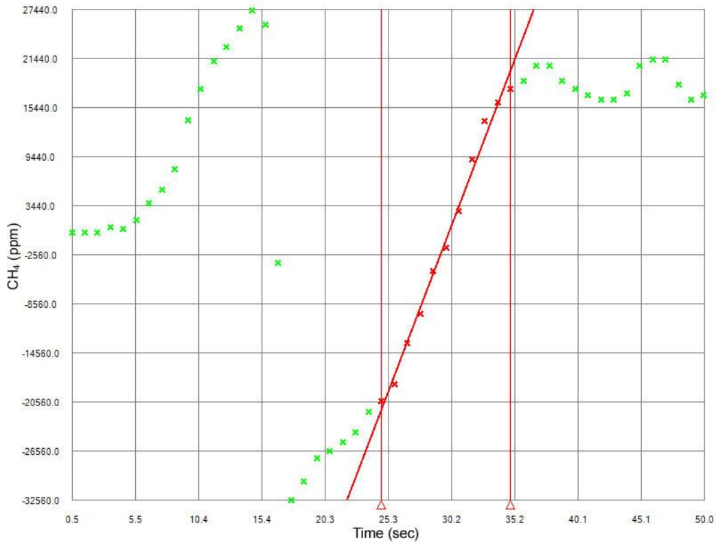
Fig. 6.2.7 Highest value of the flux recorded in Sărmășel II, M28bis
