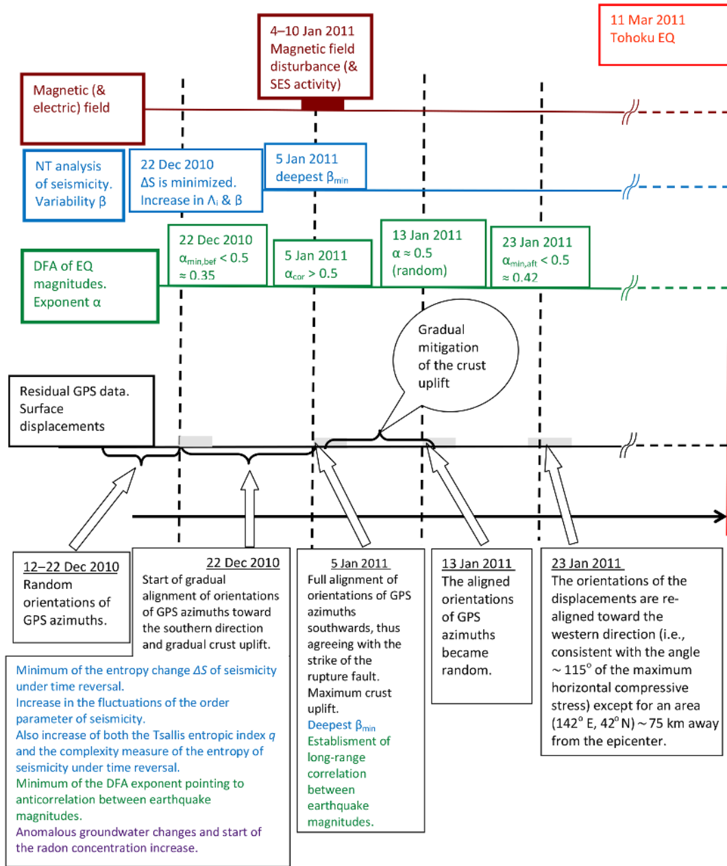
Figure 3. Schematic diagram that compiles the multidisciplinary changes before the Tōhoku EQ. Period of observations: from 12 December 2010 until 23 January 2011. The black text describes the observations by means of residual GPS data, the brown text describes those obtained by means of Earth’s magnetic field variations, the green text describes those obtained by detrended fluctuation analysis (DFA), the blue text describes those obtained by natural time analysis, and the purple text describes those obtained by anomalous groundwater and radon changes.
