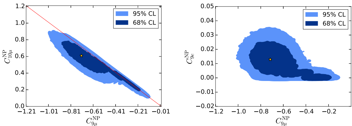
Figure 3. Allowed regions at 68% and 95% CL from the global fit for the Wilson coefficients of b \rightarrow s\ell^+\ell^- transitions. The best fit point is illustrated with a star. The red line on the left plot illustrates the correlation C_{9\mu}^{\text{NP}} = -C_{10\mu}^{\text{NP}} .
