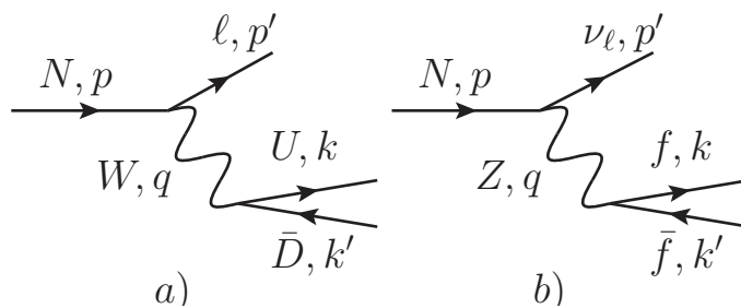
Figure 11. Diagram for the HNL decays mediated by charged a) and neutral b) currents.
