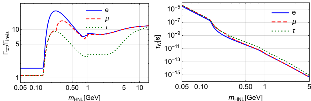
Figure 18. HNL decay width divided by the total decay width into active neutrinos eq. (3.5) (left panel) and lifetime (right panel) as a function of HNL mass. Results are given for the pure e , \mu and \tau mixings, U_\alpha = 1 .
