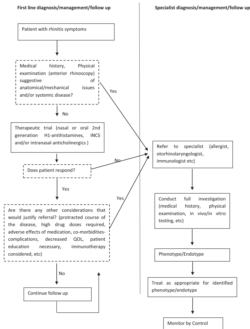
Figure 1 Simple algorithm for rhinitis management in primary and specialist care. The majority of rhinitis patients will be managed in the community; an effective mechanism for directing the right patient to the specialist is necessary.
