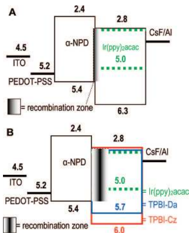
Figure 4. Energy level diagram of the PhOLEDs with TPBI (A) and TPBI-Cz and TPBI-Da (B). Plausible charge recombination-exciton generation zone is also shown. The HOMO-LUMO levels of TPBI are referred to the values in the literature, 16c and those of new host materials are derived from the electrochemical (DPV) data and corrected using the TPBI levels known from the literature. 16c
