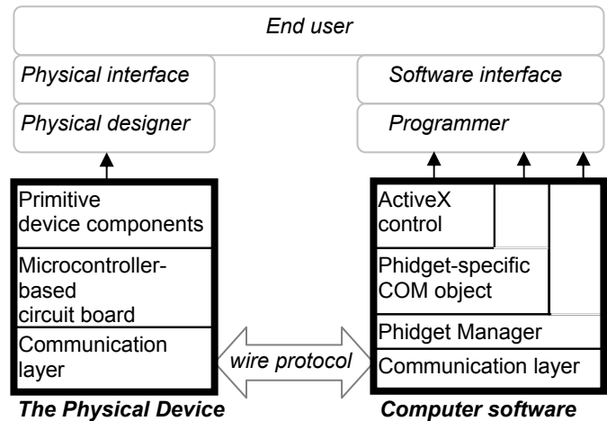
Figure 5. Phidget Architecture
