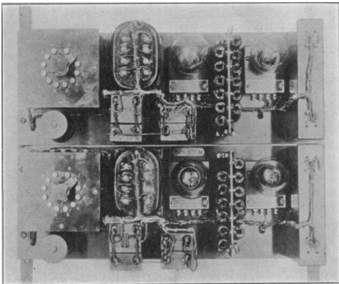
FIG. 25—ASSEMBLY OF FOUR-WIRE REPEATER APPARATUS
