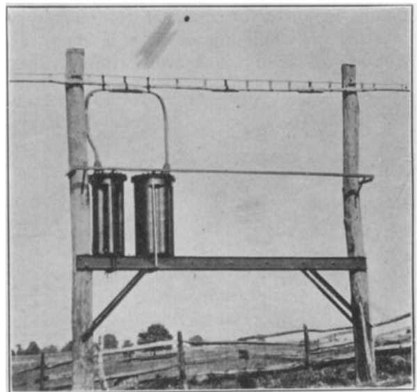
FIG. 16—LOADING FIXTURE
