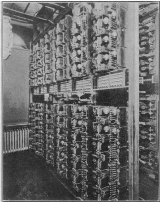
FIG. 24—GROUP OF REPEATERS AT READING, PA.
