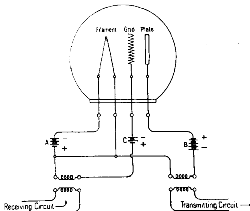
FIG. 21—VACUUM-TUBE REPEATER ELEMENT
