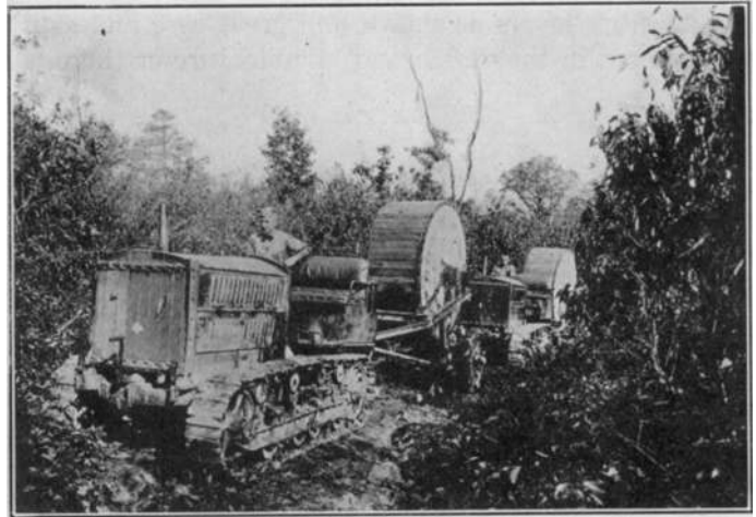
FIG. 12—TRACTORS PLACING CABLE REELS IN ROUGH COUNTRY
