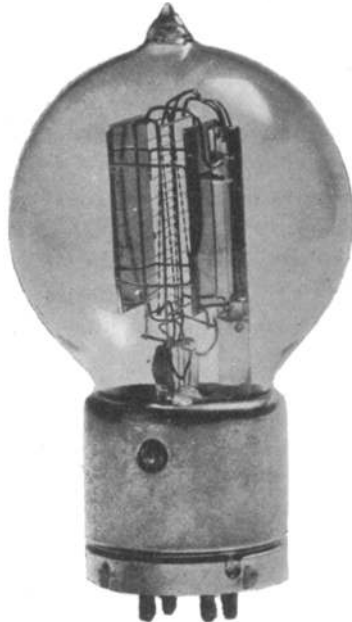
FIG. 20—VACUUM TUBE
