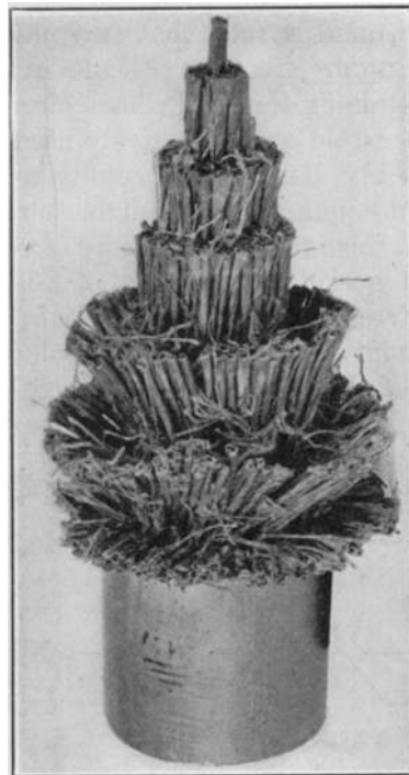
FIG. 13—PIECE OF CABLE WITH SHEATH PARTLY REMOVED
