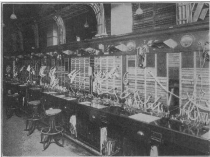
FIG. 28—TEST BOARDS
