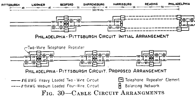
FIG. 30—CABLE CIRCUIT ARRANGEMENTS
