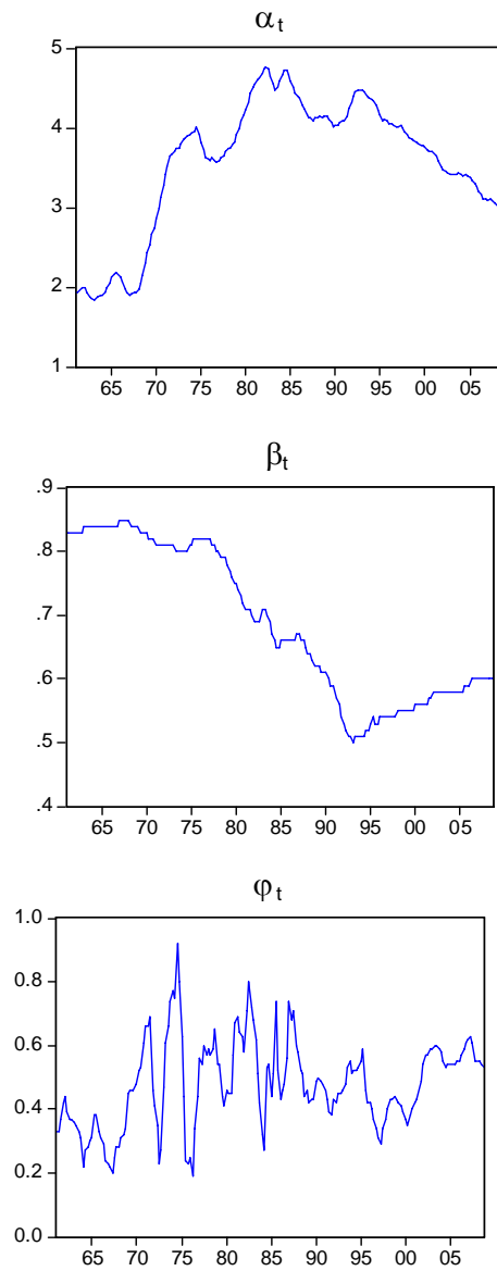
Figure 2: Time Varying Parameters
