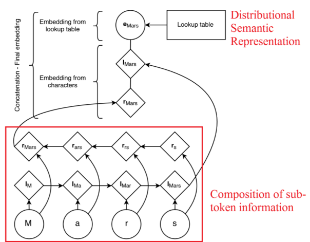
Figure 2: Type level word representations - l denotes a word prefix encoding (by forward char LSTM) while r denotes a word suffix encoding (by backward char LSTM).
