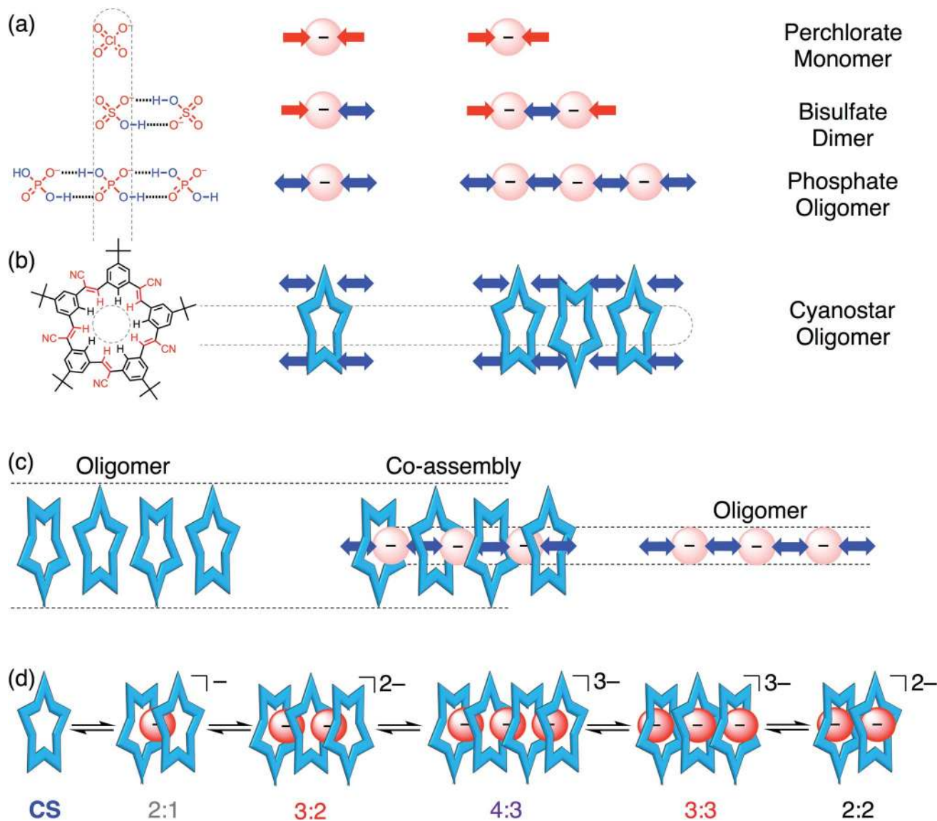
Fig. 1 (a) Anions can self-associate by hydrogen bonding to different degrees; perchlorate ( \text{ClO}_4^- ) can only accept hydrogen bonds, bisulfate ( \text{HSO}_4^- ) can also donate one hydrogen bond, and phosphate ( \text{H}_2\text{PO}_4^- ) is capable of donating two hydrogen bonds in a divergent manner. (b) Cyanostar macrocycles can capture size-matched anions and can undergo self-association. (c) The self-association of macrocycles and anions can produce co-assemblies of both. (d) Sequence of main equilibria and species present in organic solution during phosphate titration.
