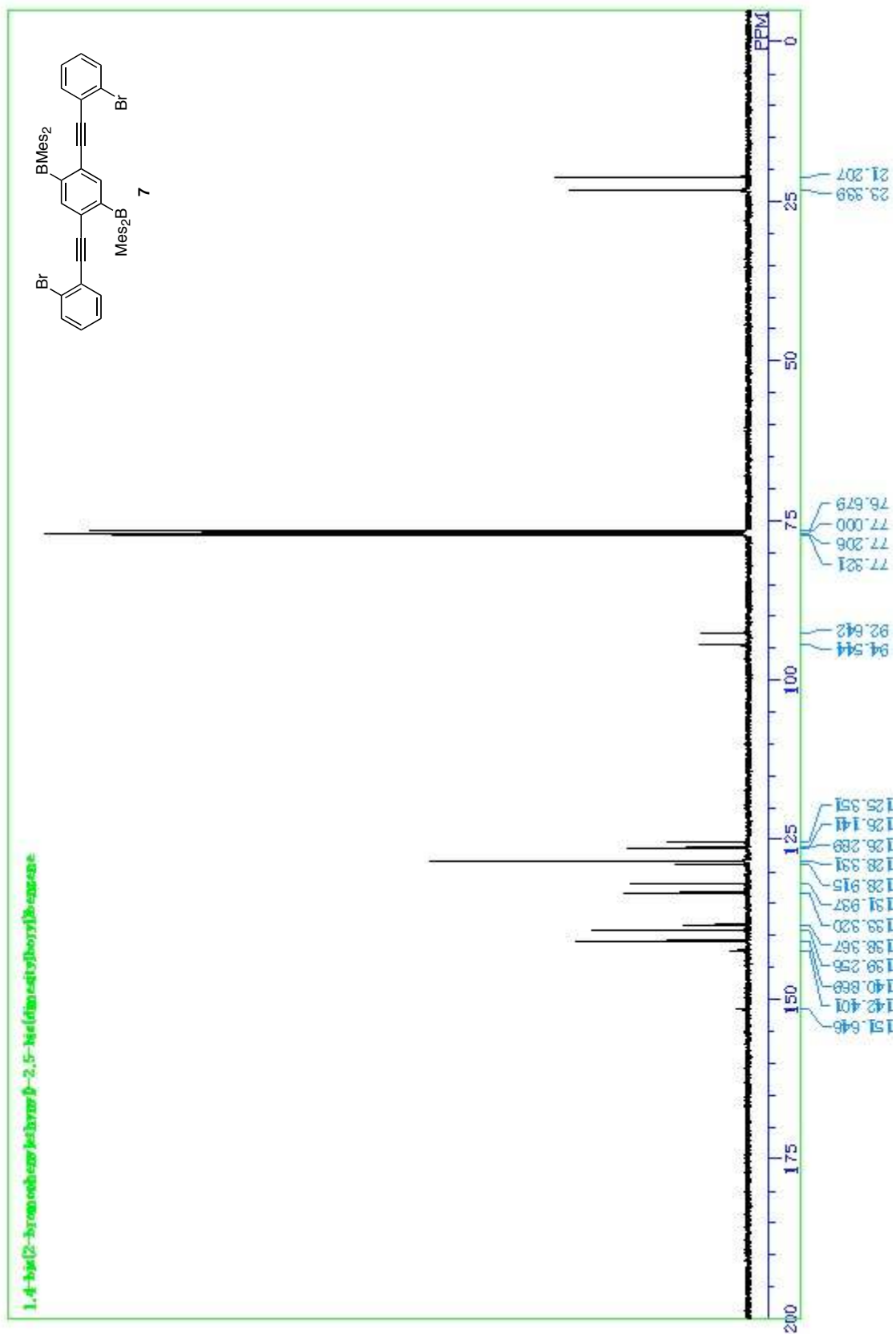
Figure S17. 13 C{ 1 H} NMR spectrum of 7 (JEOL AL-400, 100 MHz, CDCl 3 ).
