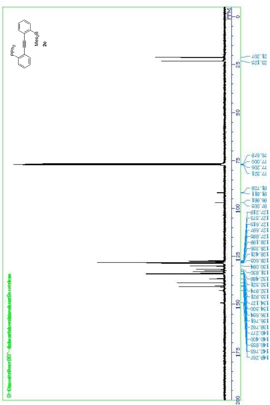
Figure S13. ^{13}\text{C}\{^1\text{H}\} NMR spectrum of 2c (JEOL AL-400, 100 MHz, \text{CDCl}_3 ).
