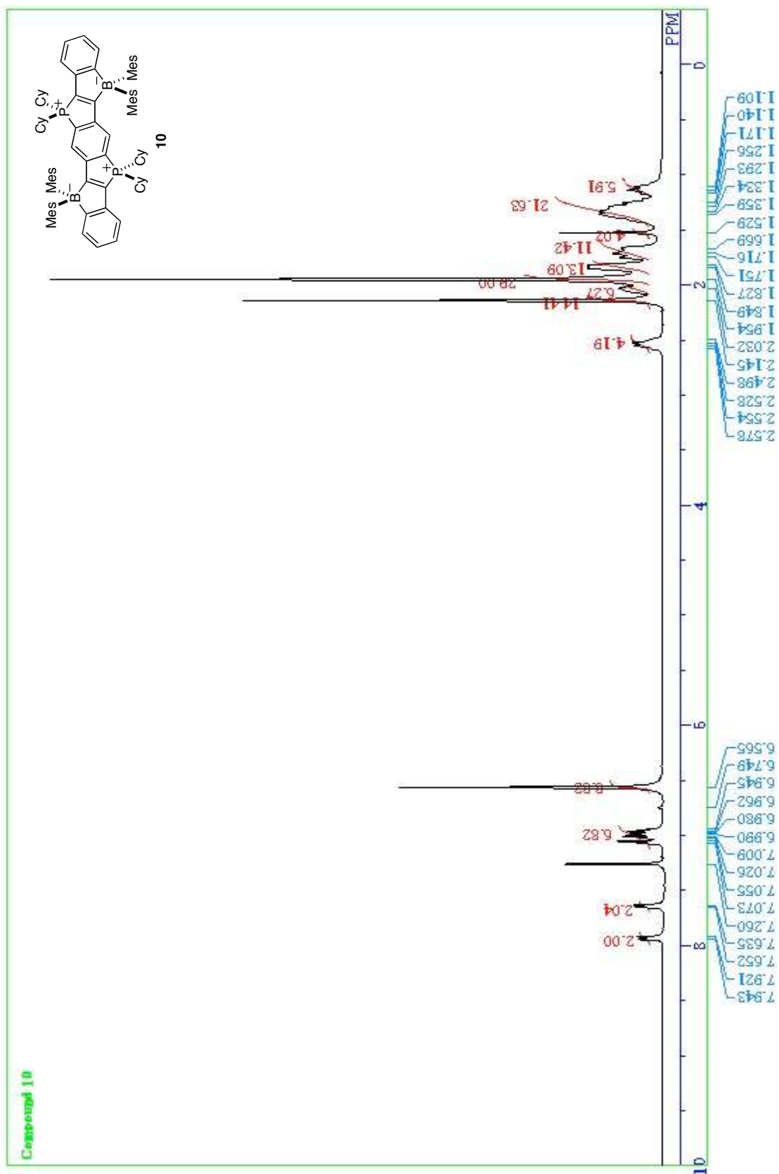
Figure S32. ^1\text{H} NMR spectrum of 10 (JEOL AL-400, 400 MHz, \text{CDCl}_3 ).
