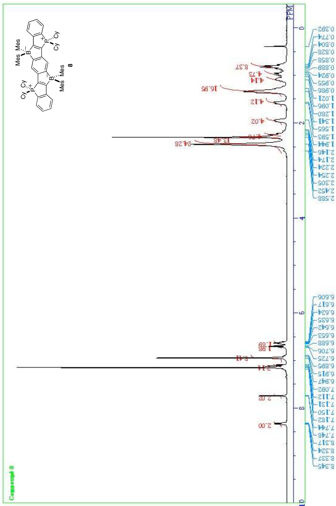
Figure S19. ^1\text{H} NMR spectrum of 8 (JEOL AL-400, 400 MHz, \text{C}_6\text{D}_6 ).
