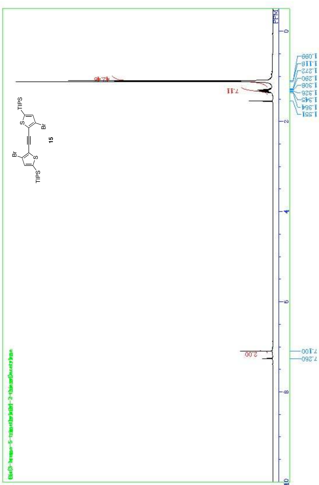
Figure S36. 1 H NMR spectrum of 15 (JEOL AL-400, 400 MHz, CDCl 3 ).
