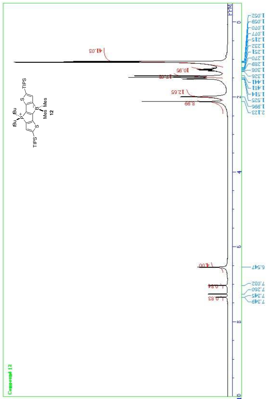
Figure S41. ^1\text{H} NMR spectrum of 12 (JEOL AL-400, 400 MHz, \text{CDCl}_3 ).
