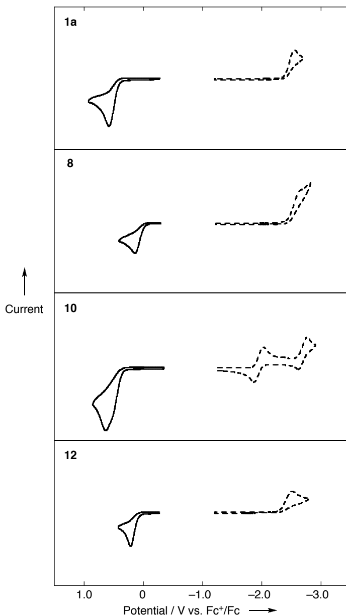
Figure S53. Cyclic voltammograms of 1a , 8 , 10 , and 12 in \text{CH}_2\text{Cl}_2 (solid line) or THF (broken line).
