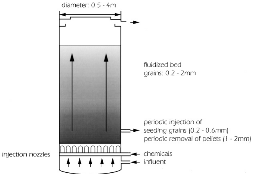
Figure 4 Cross-section through the DHV Crystalactor™. (Based on a cross-section in Reference 66.)
