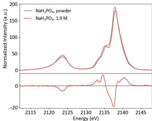
Fig. 5 Powder and solution P K \beta spectra of NaH 2 PO 4 , with difference (solution–powder).
