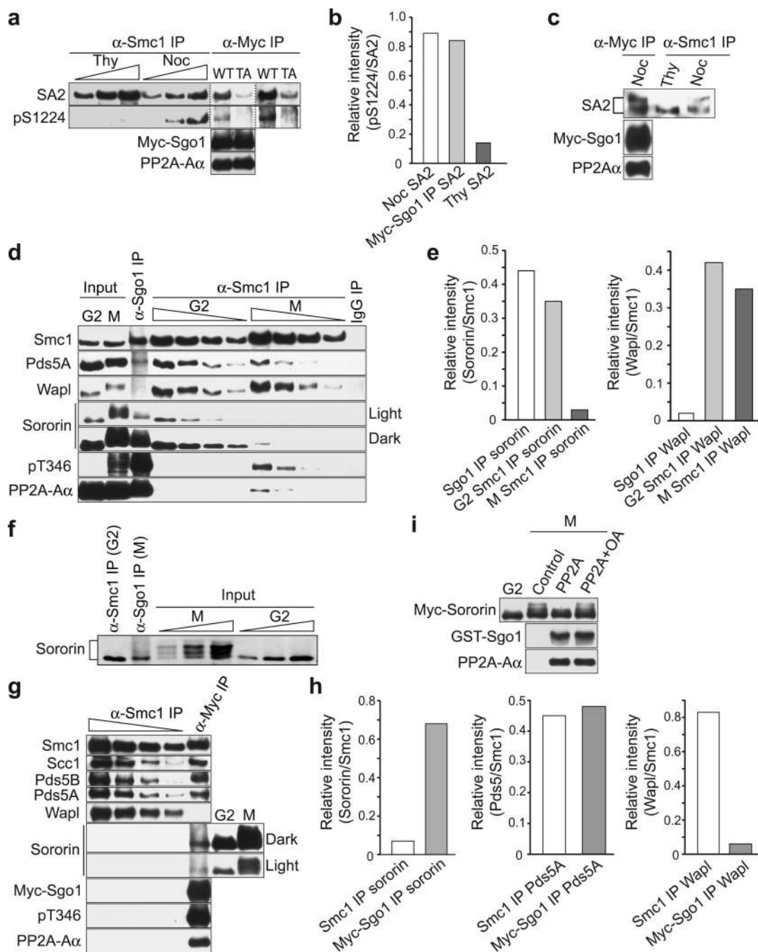
Figure 5. Sgo1-PP2A maintains cohesin-bound sororin in a hypophosphorylated state to counteract Wapl
