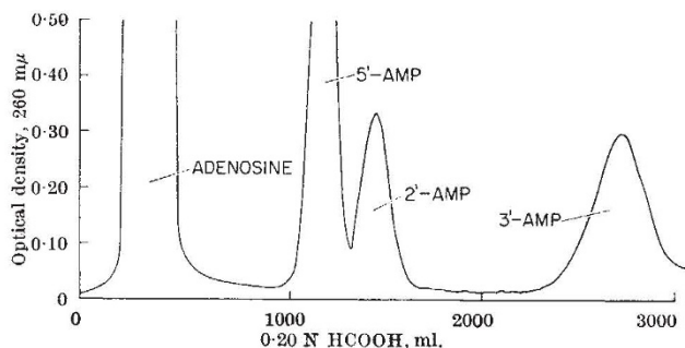
Fig. 1. Fractionation of the products of the phosphorylation of adenosine with \text{Na}_5\text{P}_3\text{O}_{10} . See Table 1 for conditions.
