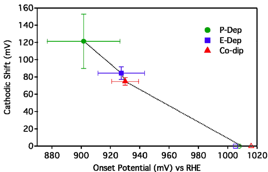
Figure S3. Average cathodic shifts plotted vs average onset potentials for Co-Pi/ \alpha -Fe 2 O 3 photoanodes prepared by photo-assisted electrodeposition (P-Dep) and electrodeposition (E-dep) of Co-Pi, and for Co 2+ / \alpha -Fe 2 O 3 photoanodes prepared by surface adsorption of Co 2+ (Co-dip) for the 12 films of Figure 5. Error bars indicate standard deviations. The open symbols represent the parent \alpha -Fe 2 O 3 photoanodes. These data show a strong correlation between the two performance metrics, with photo-assisted electrodeposition of Co-Pi leading to the lowest onset potentials and the greatest cathodic shifts.
