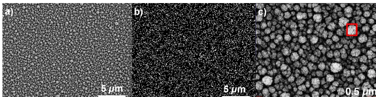
Figure S1. a) SEM image of a Co-Pi/ \alpha -Fe 2 O 3 photoanode prepared by photo-assisted electrodeposition of Co-Pi. (b) Map of the Co(K) signal intensity in the area depicted in panel (a). (c) The single nodule (of a Co-Pi/ \alpha -Fe 2 O 3 film prepared by photo-assisted electrodeposition) used in the EDX analysis of Fig. 2b. The nodule is marked with a red box.
