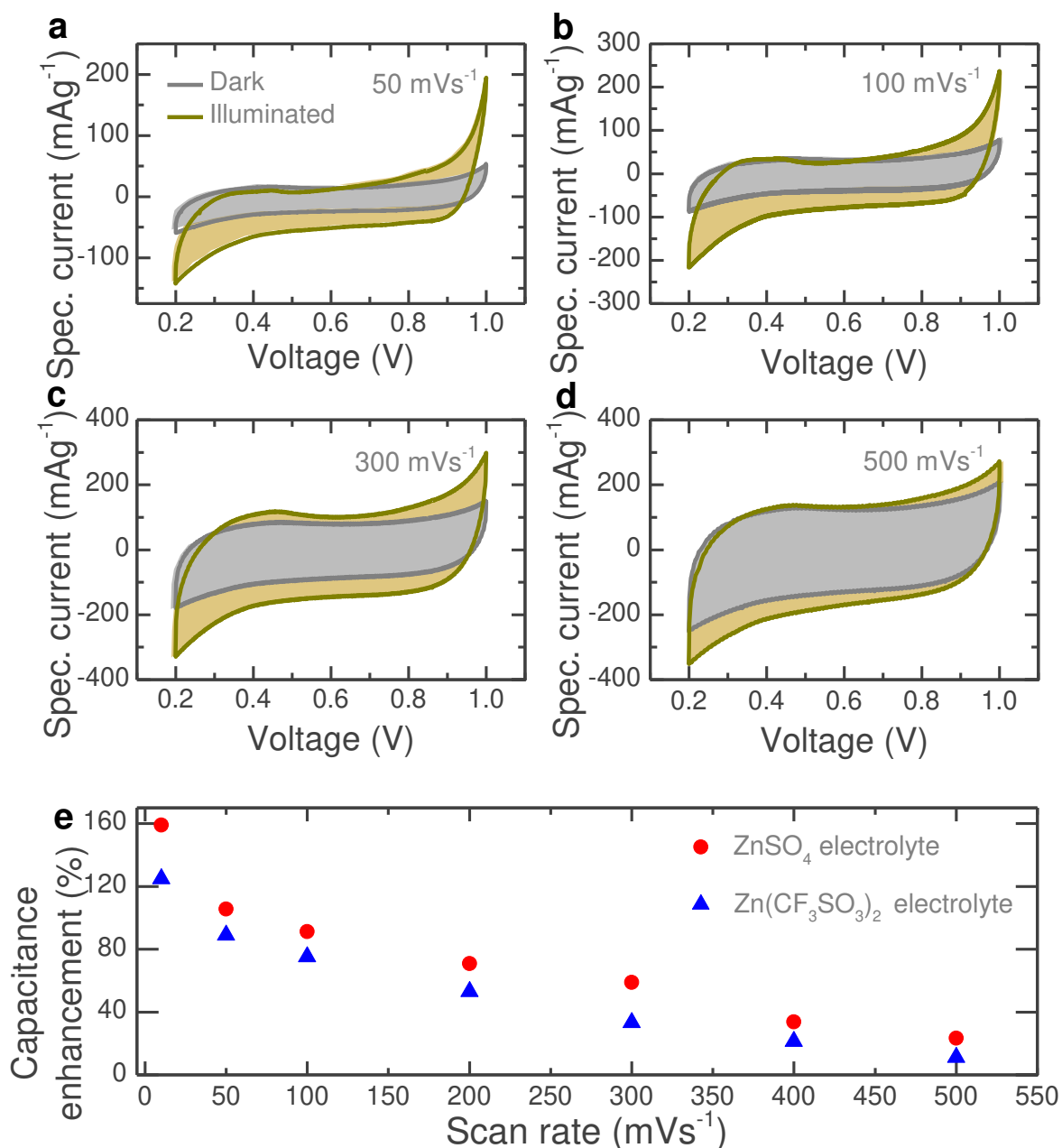
Figure 2. CV comparison of the Photo-ZIC at different scan rates of (a) 50 mVs -1 , (b) 100 mVs -1 , (c) 300 mVs -1 and (d) 500 mVs -1 in dark and illuminated ( \lambda \sim 420 nm, intensity \sim 50 mWcm -2 ). (e) Capacitance enhancement with respect to scan rate of the Photo-ZIC in ZnSO 4 and Zn(CF 3 SO 3 ) 2 aqueous electrolytes under light illumination ( \lambda \sim 420 nm, intensity \sim 50 mWcm -2 ).
