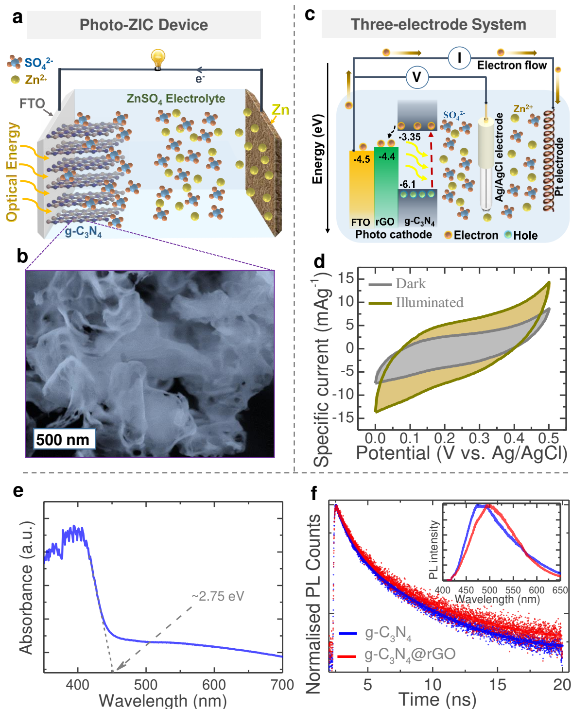
Figure 1. (a,b) Schematic illustration of 2D g\text{-C}_3\text{N}_4 cathode and Zn anode based photo-ZIC and SEM image of 2D g\text{-C}_3\text{N}_4 . (c) Schematic representation of a three-electrode experiment of
