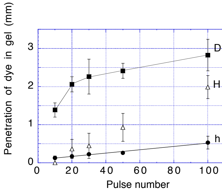
Figure 7. Effect of pulse number: Penetration of dye in clear gel against pulse number. The squares (D), triangles (H), and circles (h) present the dye distributions in their own specific directions, cf., Figure 1(b). Absorption coefficient was 300\text{ cm}^{-1} . 10–100 pulses of 60 mJ laser energy at 3 Hz were delivered through a 1000\text{ }\mu\text{m} diameter fiber. 3.5% gelatin (175 bloom) was used as the target. The fiber was located 1 mm above the gel surface. All data are mean \pm standard deviation of 5 samples.
