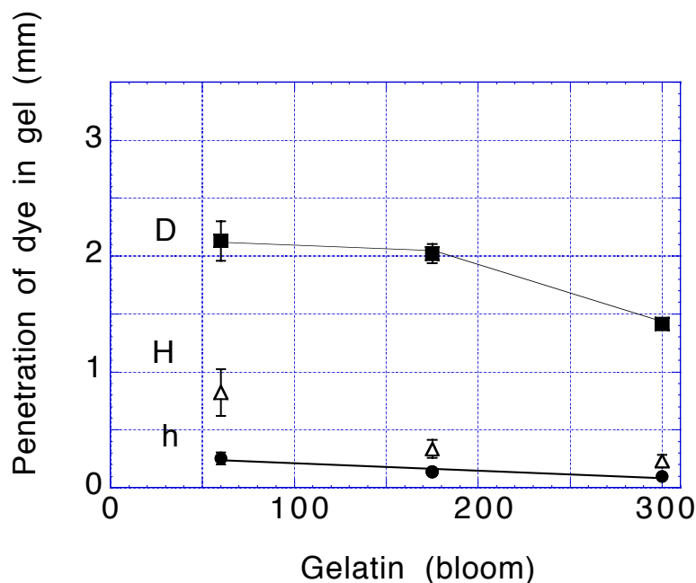
Figure 2. Effect of target materials: Penetration of dye in clear gel plotted against the gel mechanical strength. The squares (D), triangles (H), and circles (h) present the dye distributions in their own specific directions, cf., Figure 1(b). Absorption coefficient was 300\ \text{cm}^{-1} . Ten pulses of 60 mJ laser energy at 3 Hz were delivered through a 1000\ \mu\text{m} diameter fiber. 3.5% gelatin (60 bloom, 175 bloom, 300 bloom) was used as the target. The fiber was located 1 mm above the gel surface. All data are mean \pm standard deviation of 5 samples.
