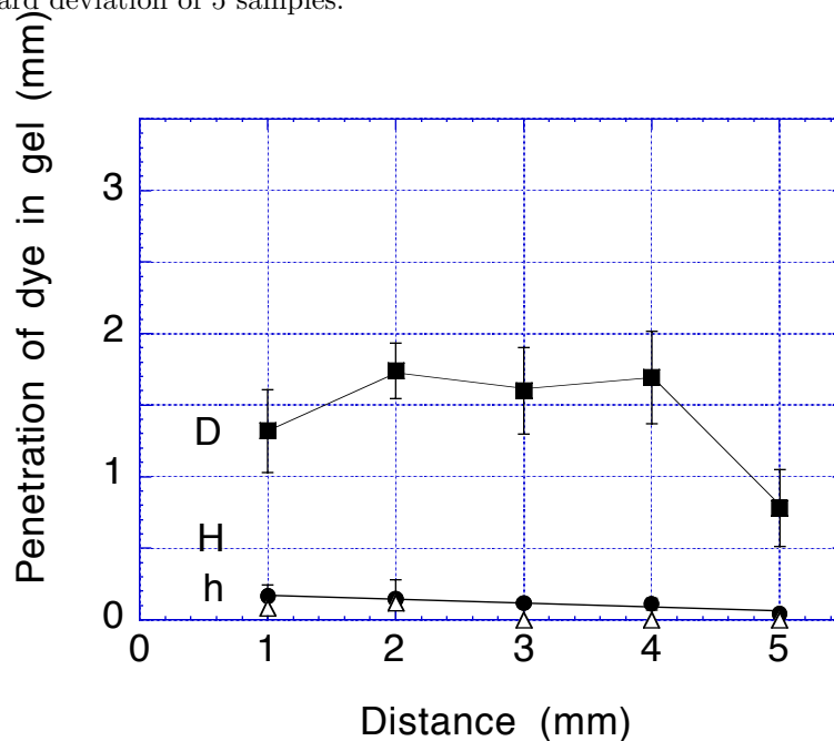
Figure 8. Effect of fiber position: Penetration of dye in clear gel as a function of the distance between the fiber tip and the gel surface. The squares (D), triangles (H), and circles (h) present the dye distributions in their own specific directions, cf., Figure 1(b). Absorption coefficient was 300\text{ cm}^{-1} . Ten pulses of 60 mJ laser energy at 3 Hz were delivered through a 1000\text{ }\mu\text{m} diameter fiber. 3.5% gelatin (175 bloom) was used as the target. The fiber was located 1–5 mm above the gel surface. All data are mean \pm standard deviation of 5 samples.
