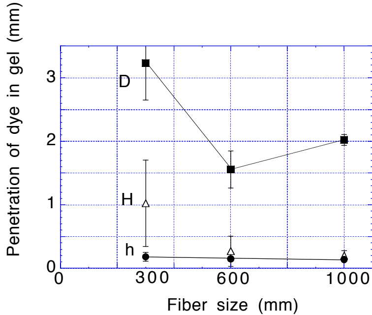
Figure 5. Effect of fiber size: Penetration of dye in clear gel plotted against fiber size. The squares (D), triangles (H), and circles (h) present the dye distributions in their own specific directions, cf., Figure 1(b). Absorption coefficient was 300\text{ cm}^{-1} . Ten pulses of 60 mJ laser energy at 3 Hz were delivered through the fibers with 300 \mu\text{m} , 600 \mu\text{m} , and 1000 \mu\text{m} diameters. 3.5% gelatin (175 bloom) was used as the target. The fibers were located 1 mm above the gel surface. All data are mean \pm standard deviation of 5 samples.
