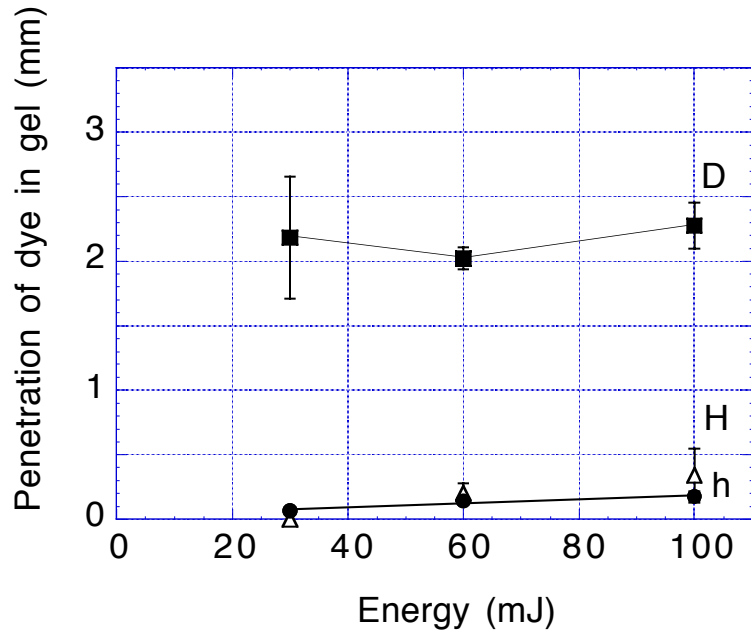
Figure 3. Effect of energy: Penetration of dye in clear gel as a function of the laser pulse energy. The squares (D), triangles (H), and circles (h) present the dye distributions in their own specific directions, cf., Figure 1(b). Absorption coefficient was 300 \text{ cm}^{-1} . Ten pulses of the laser energies (30 mJ, 60 mJ, 100 mJ) at 3 Hz were delivered through a 1000 \mu\text{m} diameter fiber. 3.5% gelatin (175 bloom) was used as the target. The fiber was located 1 mm above the gel surface. All data are mean \pm standard deviation of 5 samples.
