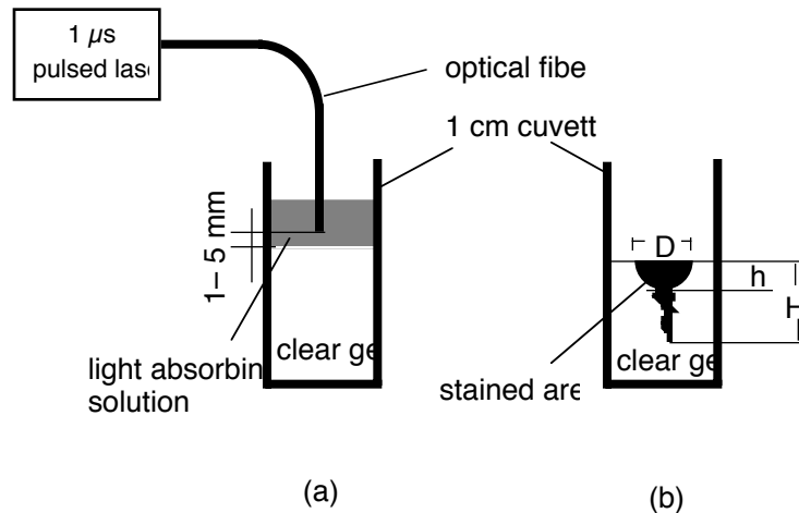
Figure 1. (a) Schematic of experimental setup. (b) Cross-section of clear gelatin after the bubble formation.
