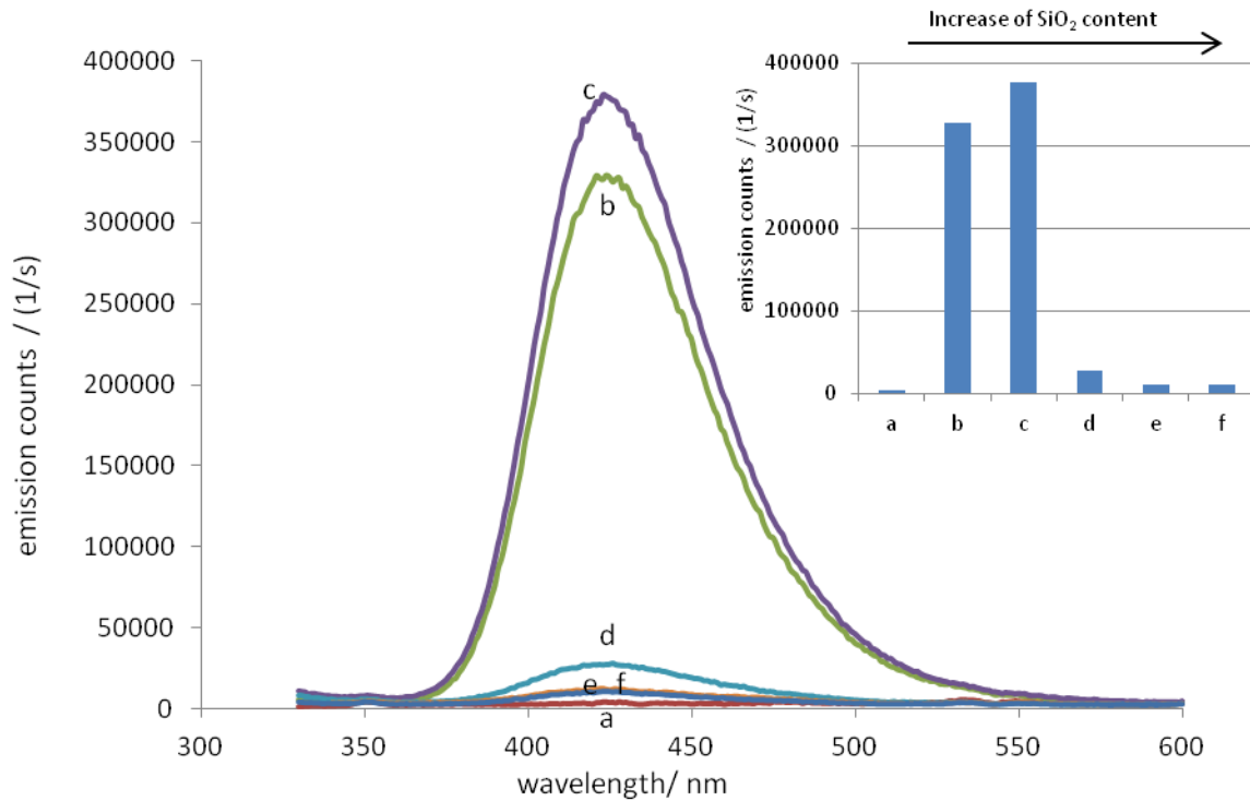
Figure 3.11. Photoluminescence spectra of polyurethane /SiO 2 -TiO 2 (A) nanocomposites varying
