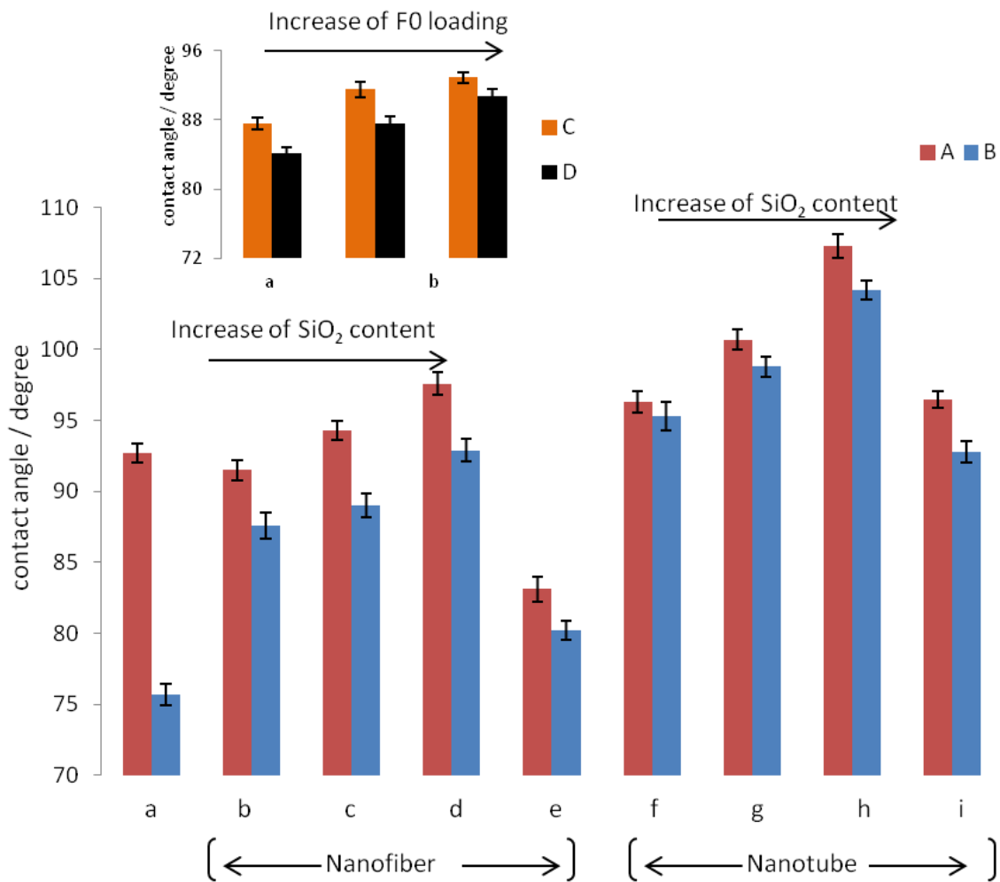
Figure 4.13. Comparison of contact angle of polyurethane coatings embedded with 5.0 mg
