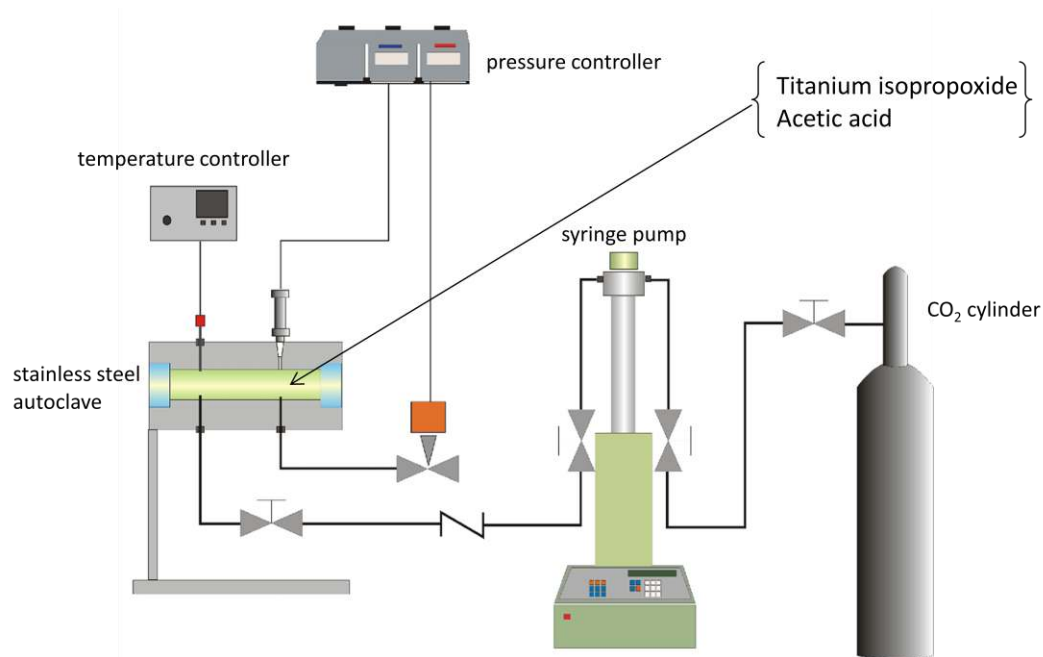
Figure 1.2. The demonstration of synthesis of TiO 2 nanofiber via supercritical CO 2 .
