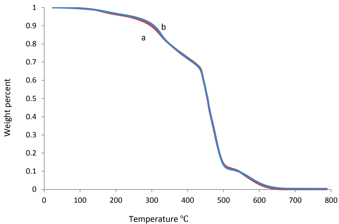
Supporting information 3.7. TGA curves of polyurethane coatings with and without nanoparticles. a: pure polyurethane; b: polyurethane with Al.
