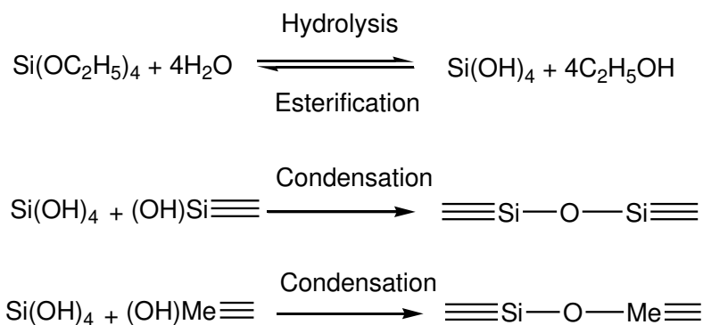
Scheme 1.4. The mechanism of modified Stöber process for silica encapsulation on metal oxide.
