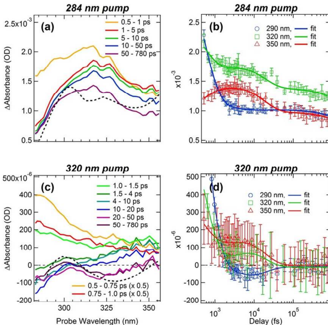
Figure 3. Averaged transient spectra and kinetic traces of aqueous [\text{Fe}(\text{CN})_6]^{4-} excited at (a,b) 284 nm and (c,d) 320 nm. The dashed black line in (a) corresponds to \epsilon_{284 \text{ nm}} and the dashed line in (c) corresponds to \epsilon_{320 \text{ nm}} , as defined in the text. Kinetic traces and fits with timescales (Table 1) derived from the full 3-dimensional dataset are shown in (b) and (d).
