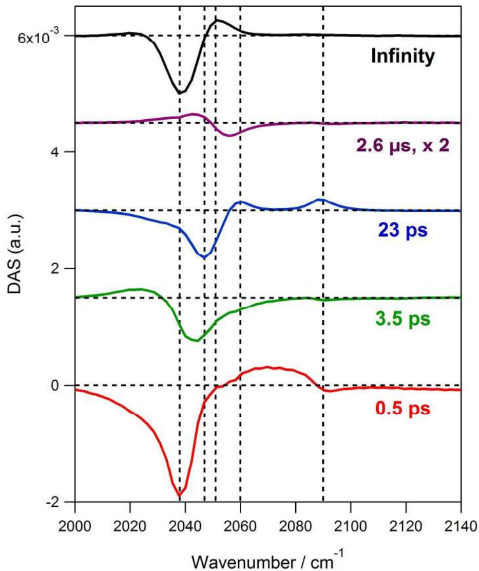
Figure 8. Decay associated spectra (DAS) obtained from the singular value decomposition of the transient IR data sets in H 2 O ( \tau_1=0.5 ps, \tau_2=3.5 ps, \tau_3=23 ps, \tau_4=\text{infinity} ).
