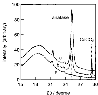
Figure 2. Representative XRD pattern of amorphous–anatase mixture of TiO 2 powders: (a) as-received amorphous, (b) mixture ( f(\text{anatase}) ca. 0.3), and (c) completely crystallized anatase. A broad peak at 2\theta = 19^\circ and small peaks at 21^\circ and 23.5^\circ are caused by vaseline used to fix the powders on an XRD sample holder. Sample b contained 20 wt % of CaCO 3 as an internal standard.
