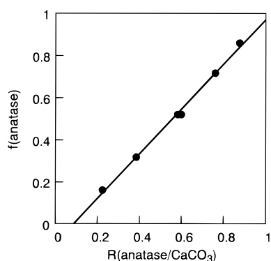
Figure 3. Calibration curve for anatase fraction as a function of peak intensity ratio of anatase TiO 2 and CaCO 3 as an internal standard. Merck TiO 2 (anatase) was used as standard anatase sample.
