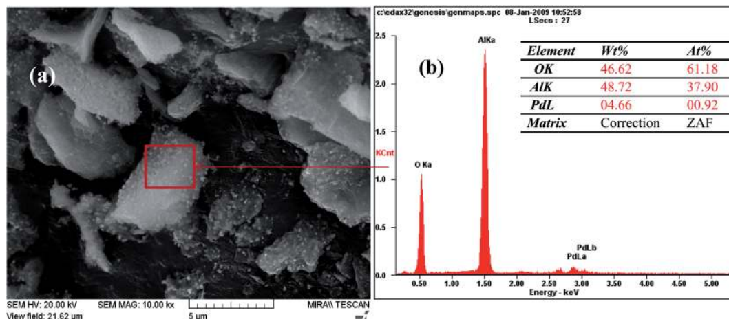
Fig. 3 EDAX analysis of Pd- \gamma -Al 2 O 3 NPs.
