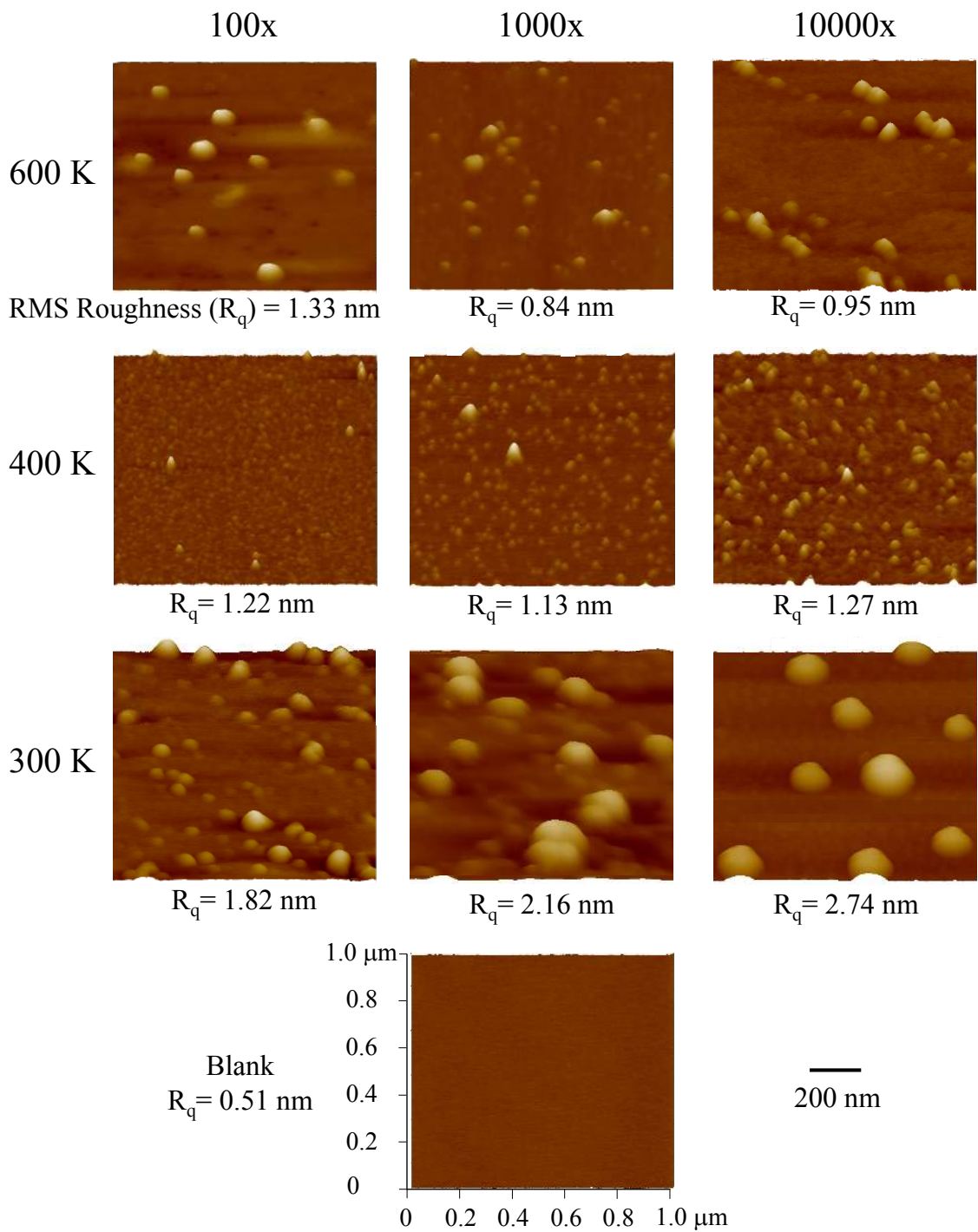
Figure 2. AFM 3D images of the particles deposited on quartz discs. Scan area is 1\ \mu\text{m} \times 1\ \mu\text{m} . Blank is the AFM image of a clean blank quartz disc. The height scale of the images is 50 nm for the 300 K and 600 K experiments, 20 nm for the 400 K experiments to better show the small particles, and also 20 nm for the blank disc. The root mean square (RMS) roughness ( R_q ) of the film ( 1\ \mu\text{m} \times 1\ \mu\text{m} ) is shown under the images. The roughness ( < 3\ \text{nm} ) indicates the films are smooth.
