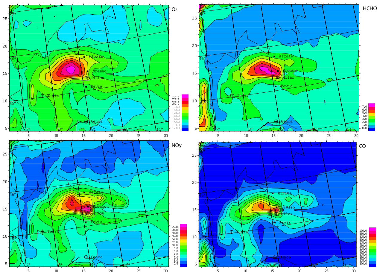
Fig. 11. Spatial distribution of O_3 , HCHO, NO_y and CO in the Po Basin, at 14:00 on 17 August. The numbers marked outside of the frames show the number of grid cells (15 km for each grid size). The longitude/latitude are marked inside of the frame. The aircraft captured the highest ozone level above 120 ppb in areas northwest of Milan city. The model results show good agreement with aircraft data.
