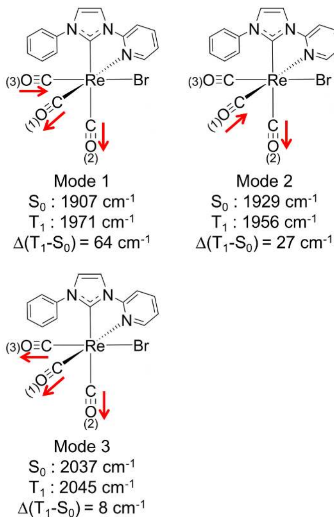
Figure 5: Vibrational phasing of the normal vibrational modes of [\text{Re}(\text{CO})_3(\text{PyImPh})\text{Br}] in the CO stretching region, their frequencies in the S_0 and T_1 states, and their differences.
