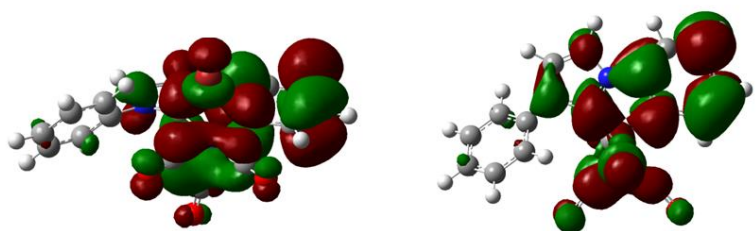
Figure 10: Molecular orbitals of [\text{Re}(\text{CO})_3(\text{PyImPh})\text{Br}] calculated by TD-DFT for the optimized geometry of the T_1 state. The two drawings of each orbital correspond to views from different directions.
