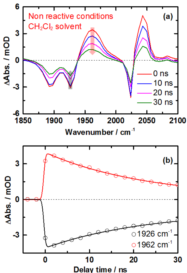
Figure 6: (a) TR-IR spectra of [Re(CO) 3 (PyImPh)Br] upon excitation at 355 nm under non-reactive conditions. (b) Temporal profiles of ΔAbs at 1962\text{ cm}^{-1} (red circles) and 1926\text{ cm}^{-1} (black circles). The red and black lines represent the corresponding fitting curves using an exponential function convolved with a Gaussian function.
