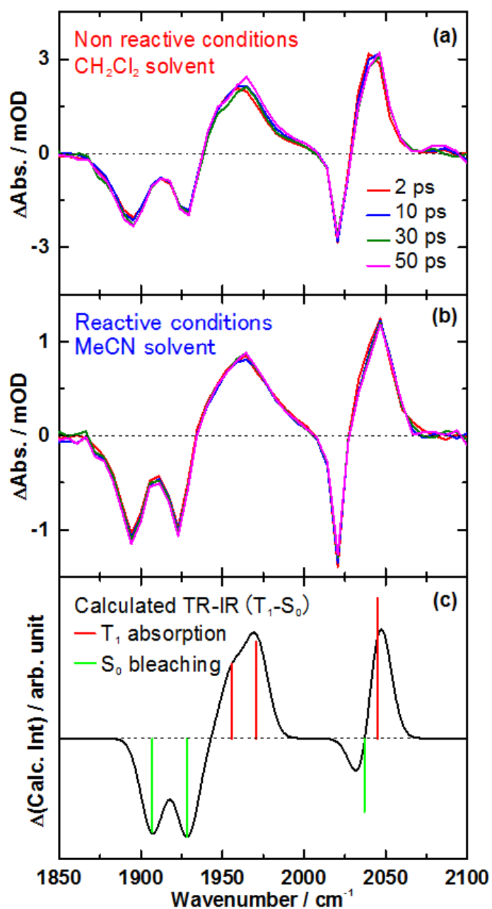
Figure 2: Temporal evolution of TR-IR spectra of [Re(CO) 3 (PyImPh)Br] after excitation at 400 nm under (a) non-reactive (in solution in CH 2 Cl 2 ) and (b) reactive (in solution in MeCN) conditions. (c) Calculated TR-IR spectrum. The bars in the spectrum provide the wavenumber and intensity of each CO stretching mode shown in Figure 5, and their colors indicate absorption of the T 1 state (red) and bleaching of the S 0 state (green).
