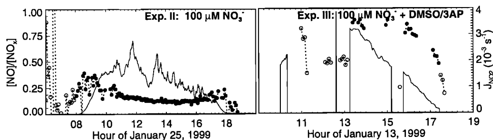
Figure 3. [\text{NO}]/[\text{NO}_x] ratios during the two experiments with \text{NaNO}_3 added. Increased scatter during periods of low mixing ratios (prior to 1000 and after 1700 on January 25, and after 1700 on January 13; see Figures 1 and 2) is the result of measurement imprecision. Symbols are as described for Figure 1.
