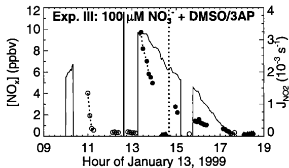
Figure 2. \text{NO}_x measurements during experiment III. Symbols are as described for Figure 1. The vertical dotted line indicates the beginning of the period used in the regression analyses of Figure 5. Nonzero J_{\text{NO}_2} values (indicated by the solid line) prior to 1300 indicate periods when the chamber was uncovered without flow (at \sim 1000 ) and was briefly uncovered with flow (at \sim 1240 ). Missing data during 1120–1205, 1405–1455, and 1630–1710 are the result of periods when the \text{NO}_x inlet was not connected to the flow chamber outlet. Missing data immediately following the time when the chamber was covered at 1510 result from the \text{NO}_x measurement cycle, which prevents accurate calculation of \text{NO}_x mixing ratios at times when mixing ratios change by large amounts.
