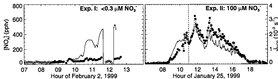
Figure 1. NO x measurements during experiments I and II. Solid circles indicate values during periods when the flow chamber was exposed to sunlight, open circles indicate observations during periods when the chamber was covered, and diamonds indicate measurements of synthetic air composition upstream of the chamber. Consecutive measurements are connected by dotted lines for clarity. The solid line indicates the downwelling component of J_{\text{NO}_2} ; J_{\text{NO}_2} is set to zero during periods when the chamber was covered. The vertical dotted line indicates the beginning of the period used in the regression analyses of Figure 4. An interruption in the rise of [NO x ] just prior to 0900 in experiment II is the result of an increase of the flow rate through the chamber to 9 sLpm, from the flow rate of 6.5 sLpm which was used overnight.
