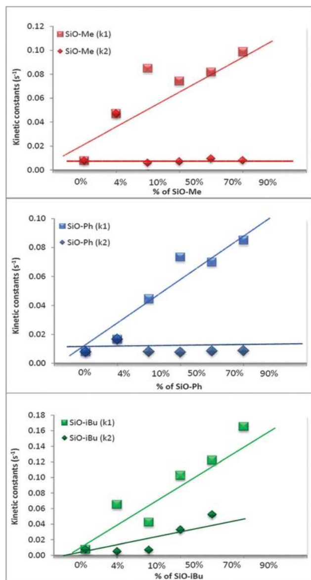
Fig. 17 Kinetic constants of the bleaching process of the photochromic naphthopyran molecules in different hybrid matrices.
