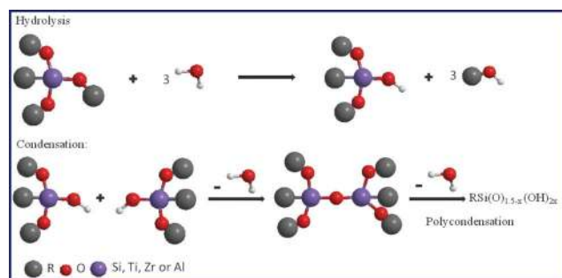
Fig. 7 Sol-gel reactions of organically modified alkoxide precursors
