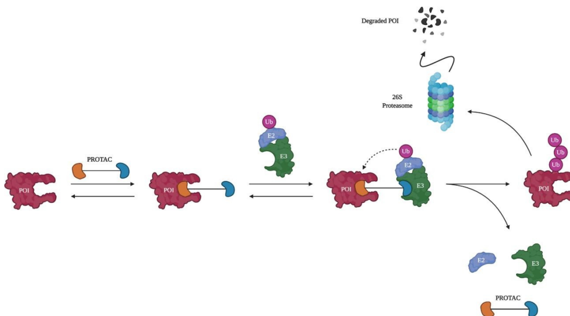
Figure 4. The mechanism of ubiquitination and subsequent protein of interest degradation by a PROTAC molecule
