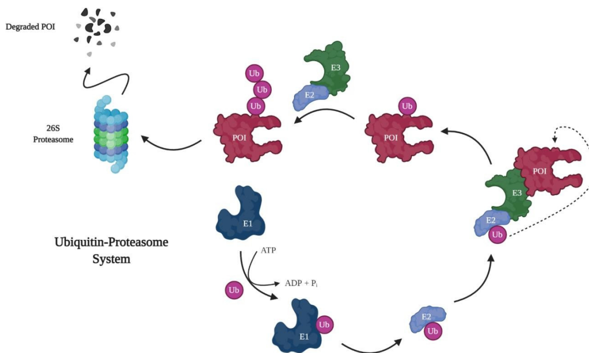
Figure 3. The mechanism of protein degradation by ubiquitin-proteasome system Slika 3. Mehanizam degradacije proteina ubikvitin-proteazom sistemom
