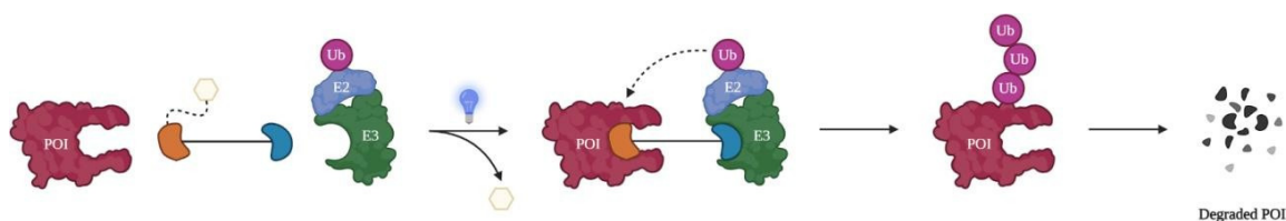
Figure 5. PROTAC releasing from pc-PROTAC after light irradiation
