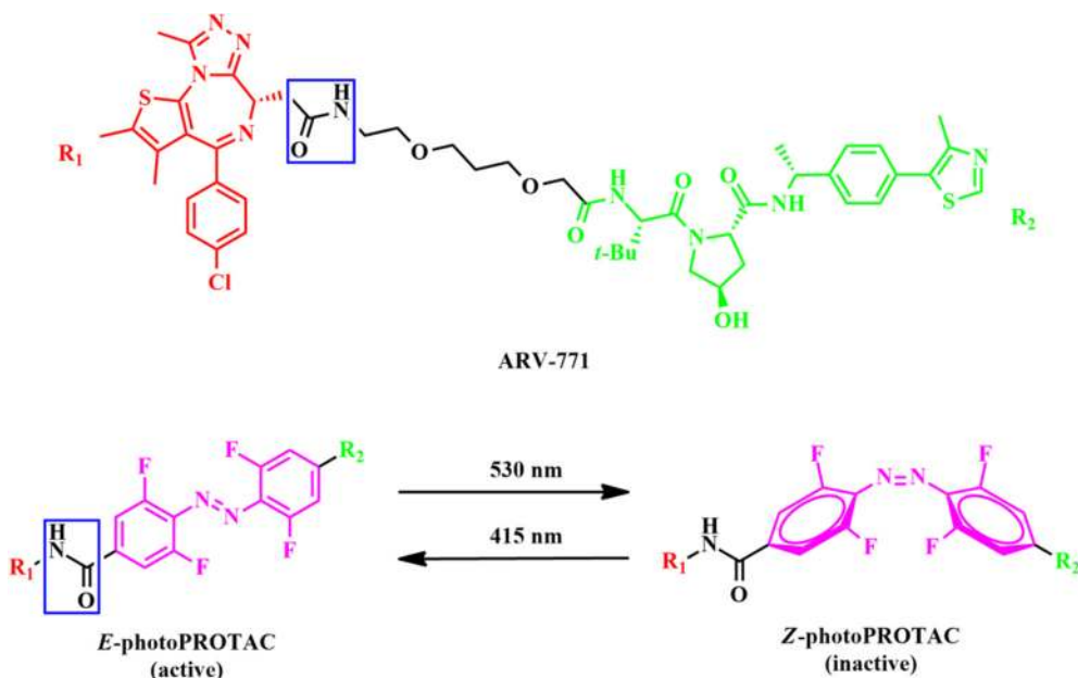
Figure 9. The chemical structure of ARV-771 as the lead structure for the generation of the photoPROTAC and its photoinduced switching Slika 9. Hemijska struktura ARV-771 kao vodećeg jedinjenja za stvaranje photoPROTAC molekula i njegov fotoindukovani prelaz
