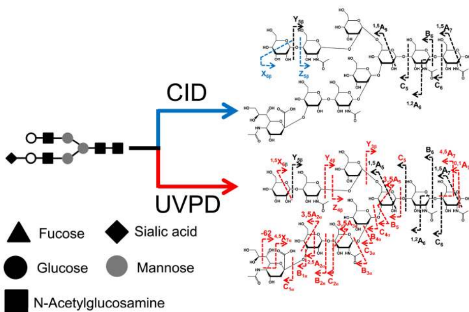
Figure 12. MS/MS fragmentation maps of deprotonated [2\text{Ant1SiA} - \text{H}]^- (a two antenna glycan from feturin, m/z 1930) by CID and 193 nm UVPD with 20 pulses. Reprinted with permission from reference 133. Copyright American Chemical Society 2011.
