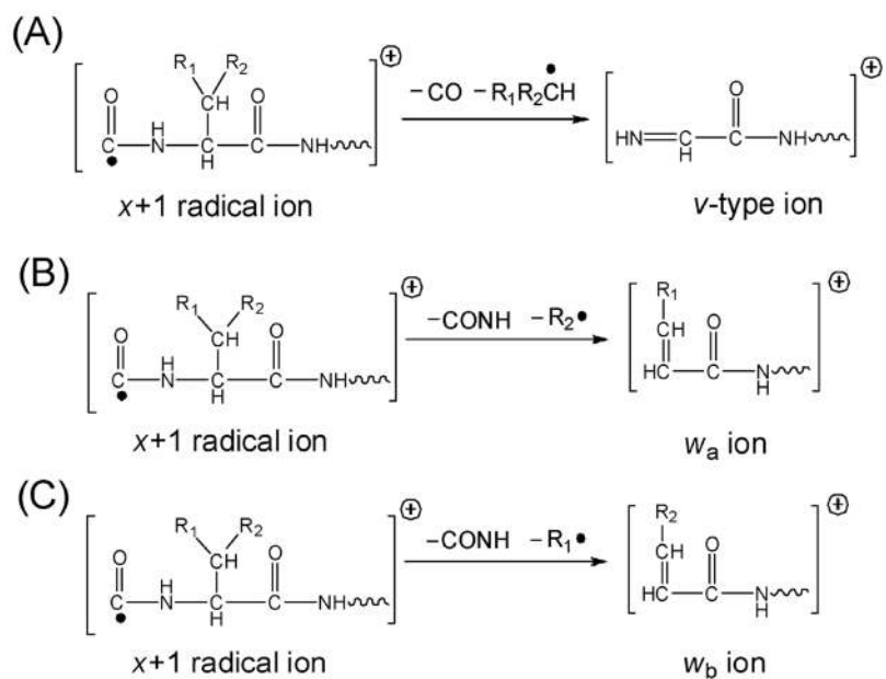
Figure 9. Formation of \nu and w ions upon UVPD. Reprinted with permission from reference 121. Copyright American Chemical Society 2010.
