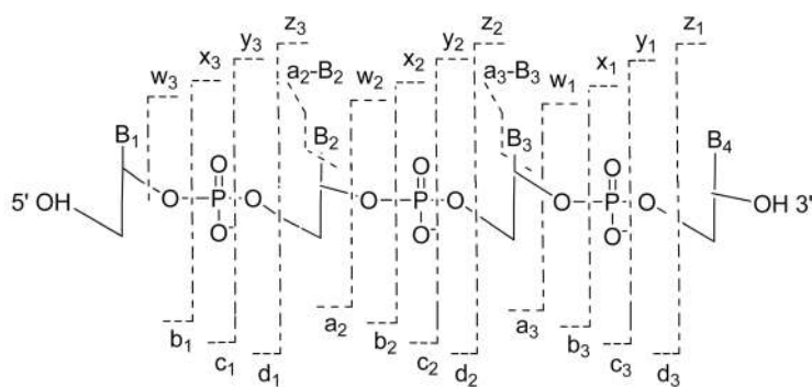
Oligonucleotide Fragmentation Nomenclature
