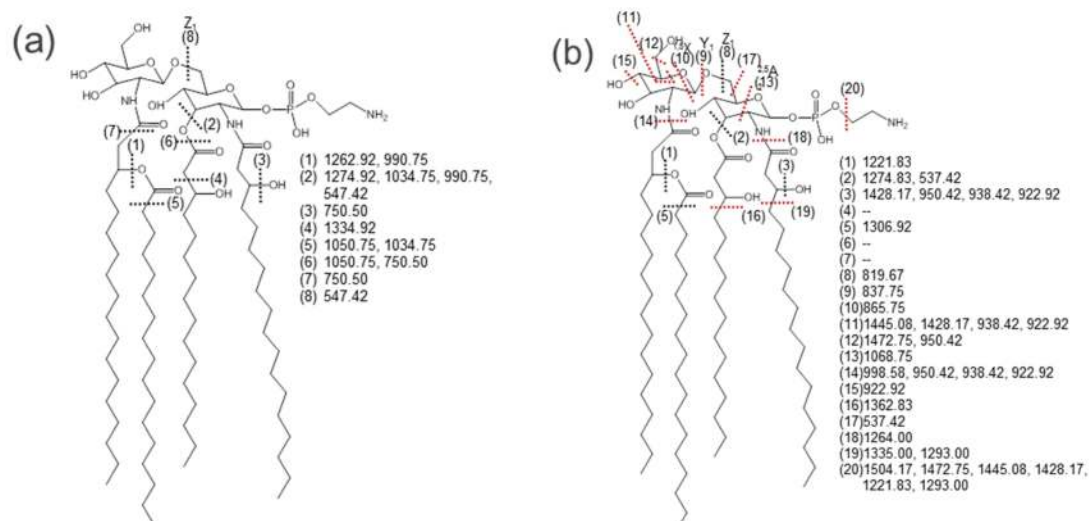
Figure 13. Fragmentation maps of H. pylori lipid A (MW 1548.2) by (a) CID, 1-, and (b) 193 nm UVPD, 1-. Dashed lines represent cleavage sites and are matched with the m/z values to the right of each structure. Key cleavages seen for UVPD that were not observed for CID are marked with red lines. Reprinted with permission from Reference 130. Copyright American Chemical Society 2011.
