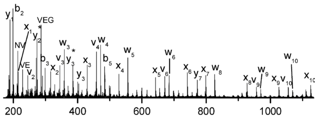
Figure 10. Photodissociation mass spectrum of protonated peptide VVVEGVNVITK* (ionized by MALDI) from a tryptic digest of ribosomal protein L24 after guanidination of the digest (where K* represents guanidinated lysine). The observation of the v 3 and w 3 side-chain loss ions confirm that the third residue from the C-terminus of the peptide is isoleucine, not leucine. Adapted from reference 121. Copyright American Chemical Society 2010.
