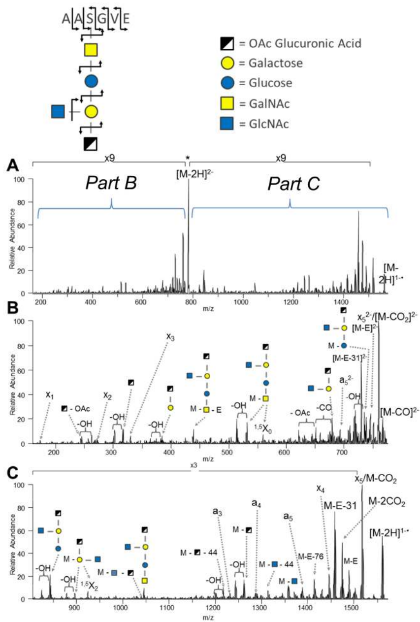
Figure 17. UVPSD of the doubly deprotonated glycopeptide AAS(glycan)GVE from Acinetobacter baumannii Ompa/MotB. Reprinted with permission from reference 142. Copyright American Chemical Society 2013.
