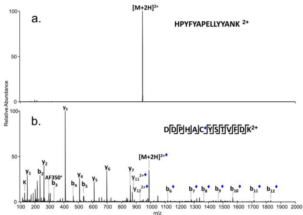
Figure 27. 351 nm UVPD mass spectra of tryptic BSA peptides (a) HPYFYAPELLYYANK 2+ and (b) Alexa Fluor 350 conjugated DDPHACYSTVFDK 2+ following 351 nm photoirradiation with 10 pulses at 3 mJ. Reprinted with permission from reference 62. Copyright American Chemical Society 2013.
