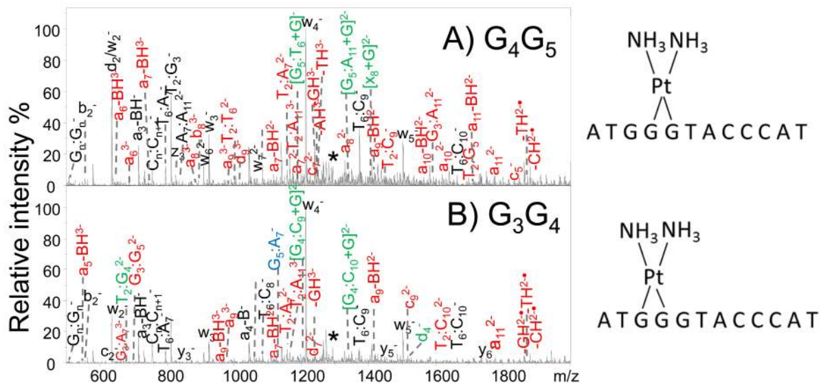
Figure 4. IRMPD spectra for (A) the G 4 G 5 cisplatin cross-link (3-, m/z 1286.7) and (B) the G 3 G 4 cisplatin cross-link (3-, m/z 1286.7) of d(ATG GGT ACC CAT) ( M_r of the cross-link product is 3863.2 Da). Fragment ions in red and in green contain the Pt modification. Fragment ions in black and in blue are the Pt-free fragments. Unique fragments for each adducts that allowed them to be identified are labeled in green and blue. Precursor ions are noted with an asterisk. Reprinted with permission from Reference 92. Copyright Springer 2014.
