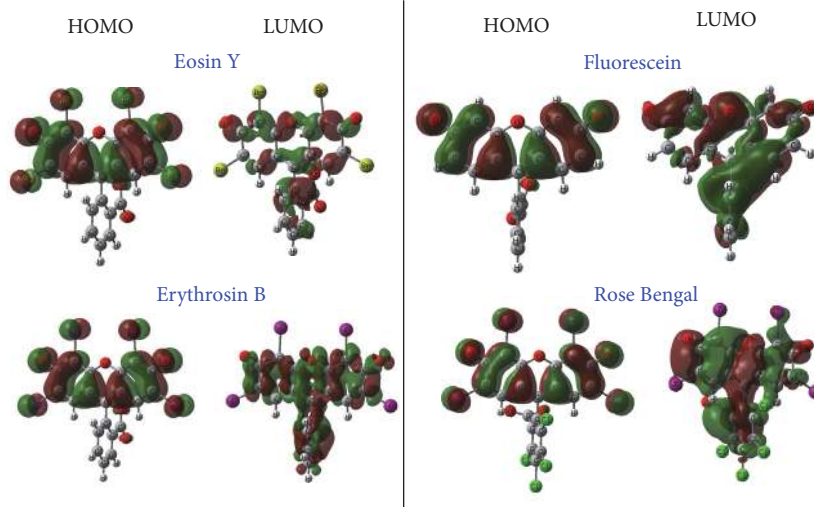
FIGURE 3: Plots of frontier orbitals (HOMO and LUMO) for the four xanthene dyes studied.
