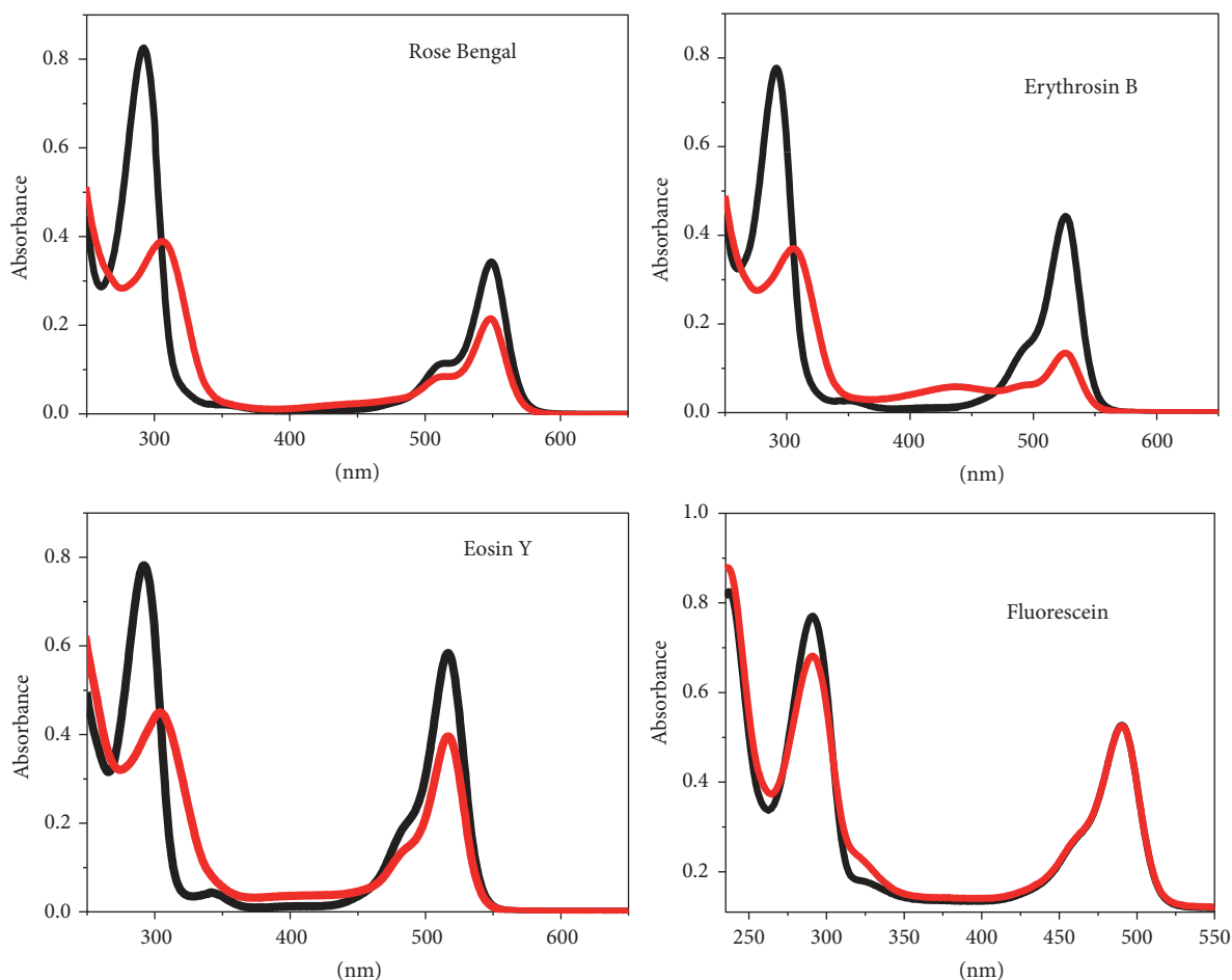
FIGURE 2: Absorption spectra of solutions containing uric acid ( 10 \mu\text{g mL}^{-1} ) and dye ( 5 \mu\text{g mL}^{-1} ) dissolved in PBS before (black) and after (red) the irradiation with LED. The absorption spectra show the decrease of the band in 292 nm attributed to the acid uric photooxidation.
