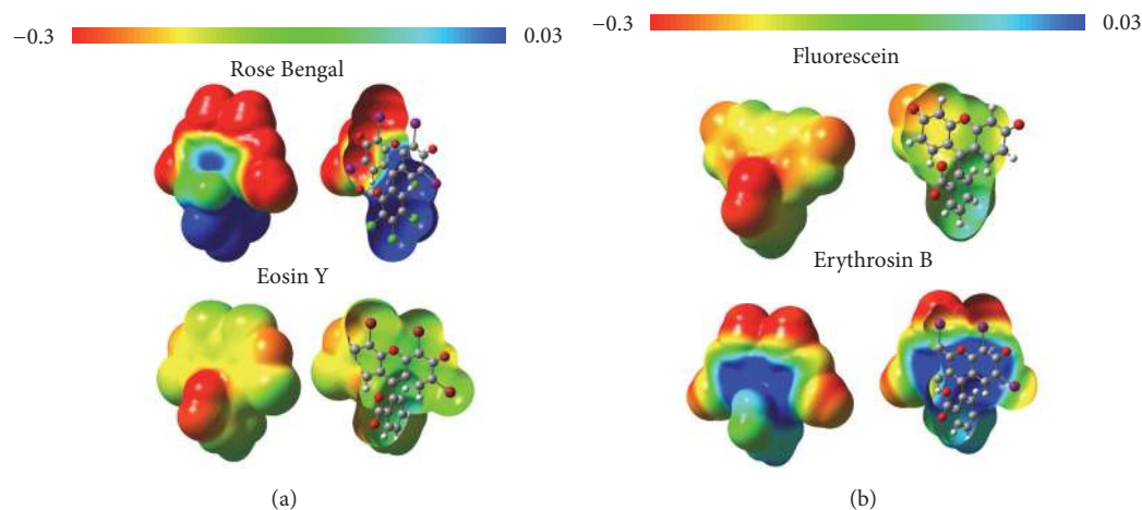
FIGURE 4: Molecular electrostatic potential of each xanthene dye (isovalue of 0.0004 a.u.). The right-side view shows the front of the solid surface, and the left-side view shows the back of the surface and displays its molecular disposition. The regions in red refer to areas with an electrophilic character, while the regions in blue are areas with a nucleophilic nature. A different case is the area in green which is related to neutral regions.
