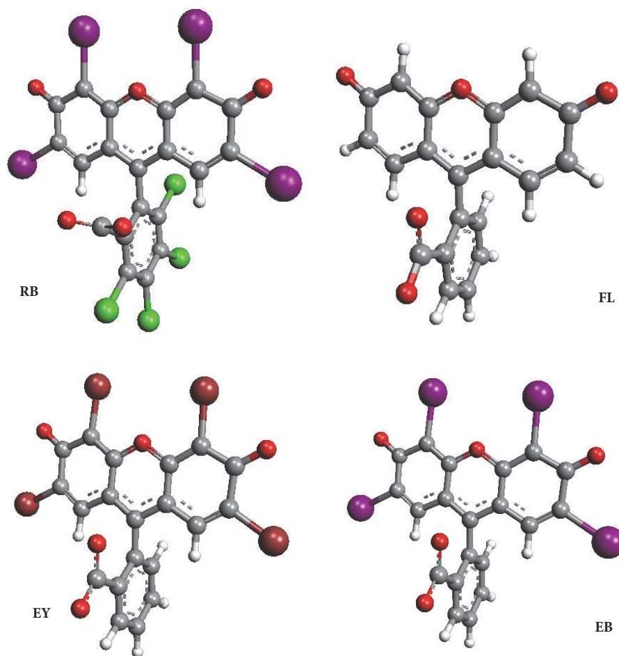
FIGURE 1: The optimized structures of the four xanthene dyes with B3LYP/6-31+G(d). The xanthene dyes: Rose Bengal ( RB ), erythrosin B ( EB ), eosin Y ( EY ), and fluorescein ( FL ).
