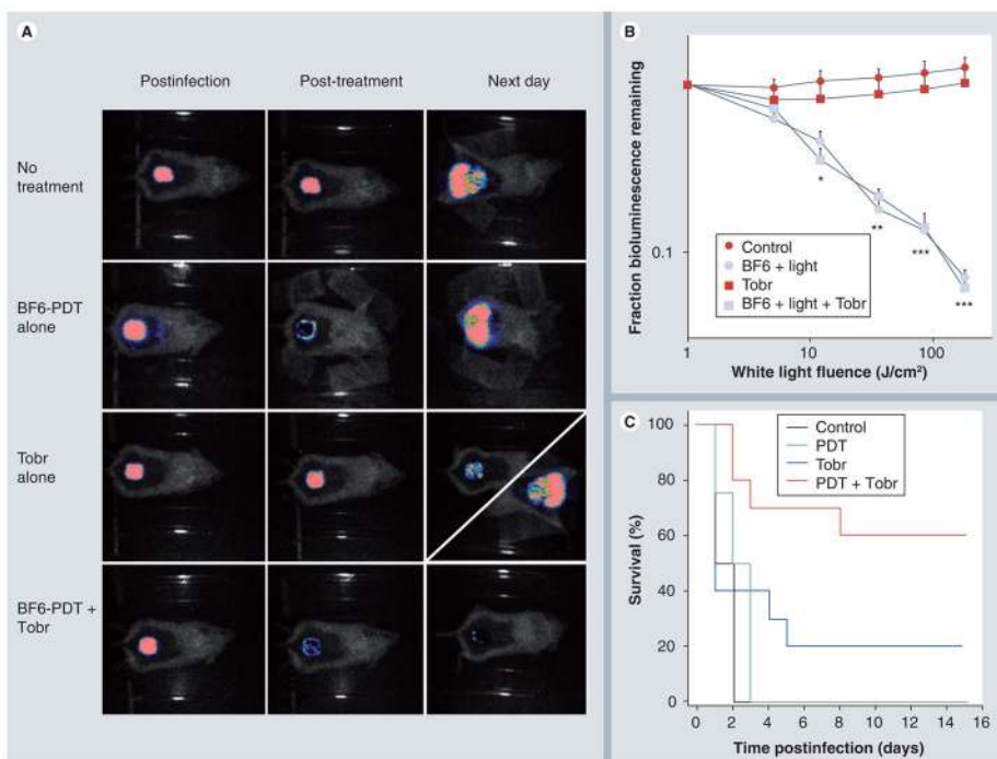
Figure 4. BF6-PdT and tobramycin treatment of Pseudomonas aeruginosa wound-infected mice (A) Representative bioluminescence images of P. aeruginosa -infected mice (captured immediately postinfection, immediately post-treatment and 24 h post-treatment), receiving: no treatment (top row); treated with BF6-PDT alone (180 J/cm 2 ; second row); treated with Tobr alone (6 mg/kg for 1 day; third row, diagonal panel 24 h post-treatment shows two possible outcomes); and treated with a combination of BF6-PDT and 1 day Tobr (bottom row). (B) Quantification of luminescence values from bioluminescence images (not shown) obtained during the PDT process, or at equivalent times for non-PDT mice. * p < 0.05; ** p < 0.01; *** p < 0.001; BF6 plus light (with and without Tobr) versus BF6 in dark and versus Tobr alone. (C) Kaplan–Meier survival curves for the groups of mice in Figure 4A; no treatment control (n = 10); PDT alone (n = 12); Tobr alone (n = 2); PDT plus Tobr (n = 10). PDT: Photodynamic therapy; Tobr: Tobramycin.
