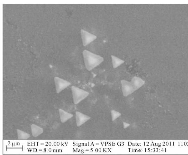
Figure 2. SEM image of fabricated TiO 2 .
