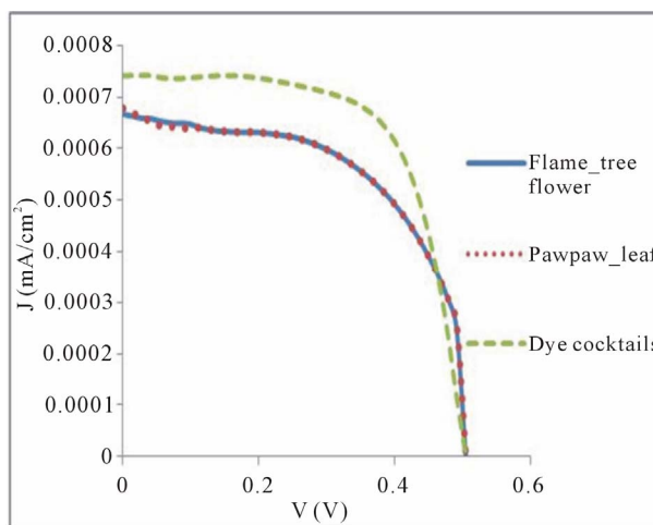
Figure 6. J-V characteristics of DSSCs with flame tree flower, pawpaw leaf and combination extracts dye.
