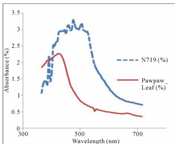
Figure 4. Absorption spectra of N719 dye and Pawpaw leaf.
