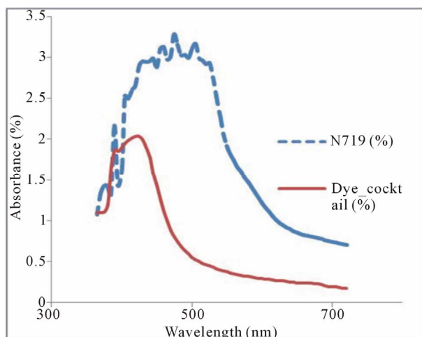
Figure 5. Absorption spectra of N719 dye and cocktail dye.
