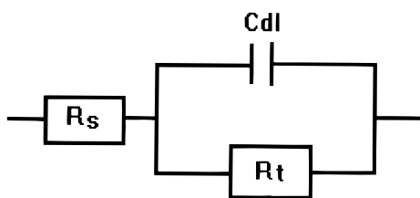
Figure 9. The equivalent circuit of the photoelectrochemical degradation of SSal.
