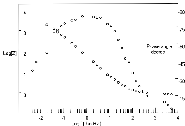
Figure 8. EIS Bode plots of SSal photoelectrochemical degradation N _2 -purged, other experimental conditions are the same as in Figure 7.
