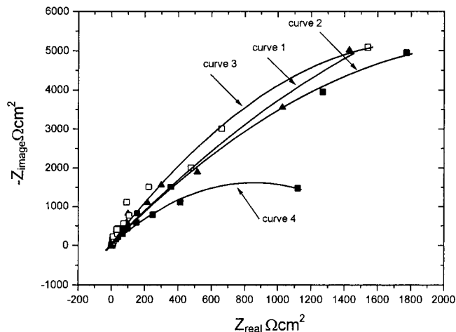
Figure 10. EIS Nyquist plots of SSal photoelectrochemical degradation: SSal concentration = 5.0 \times 10^{-4} mol L ^{-1} . Curve 1, dark, no bias; curve 2, dark, bias = 50 mV; curve 3, illumination, no bias; curve 4, illumination, bias = 50 mV.
