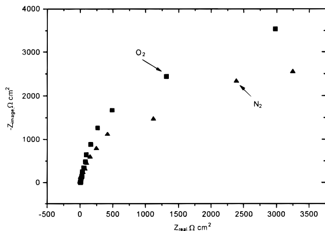
Figure 7. EIS Nyquist plots of SSal photoelectrochemical degradation: SSal concentration = 5.0 \times 10^{-4} mol L ^{-1} , external bias = 50 mV.
