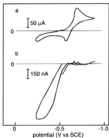
Figure 7. (a) Dark current and (b) photocurrent vs potential curves of a Q-PbS particle layer in a solution containing 2 mM MV^{2+} and 0.5 M NaClO_4 . The potential range was between -0.23 and -0.9 V; sweep direction was -0.52 \rightarrow -0.9 \rightarrow -0.23 \rightarrow -0.52 V. The other experimental conditions were the same as those in Figure 2.
