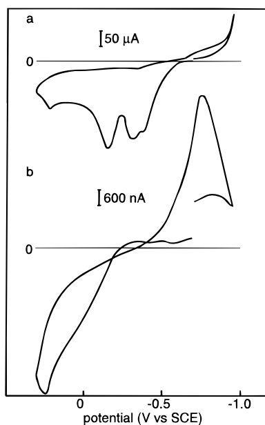
Figure 8. (a) Dark current and (b) photocurrent vs potential curves of a Q-PbS particle layer in a solution containing 2 mM S_2^{2-} and 0.5 M NaClO_4 . The potential range was between 0.3 and -0.95 V; sweep direction was -0.7 \rightarrow 0.3 \rightarrow -0.95 \rightarrow -0.7 V. The other experimental conditions were the same as those in Figure 2.
