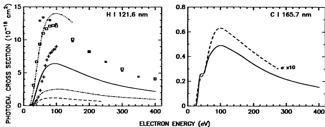
FIG. 6. Comparison of excitation functions for H I and C I transitions in dissociative excitation of methane molecules. All photoemission cross sections are in 10^{-18} cm 2 . Measurements shown are: ■ Vroom and de Heer (1969a), ·· Sroka (1969b), ···· McGowan et al. (1969), --- Morgan and Mentall (1974), □ Möhlmann et al. (1978), + Orient and Srivastava (1981), and — Pang et al. (1987).
