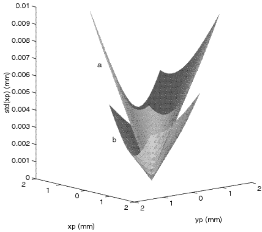
Figure 4. Effect of three-dimensionality (step height H ) on topology of the objective function near the minimum point. (a) H = 6 in, (b) H = 2 in.
