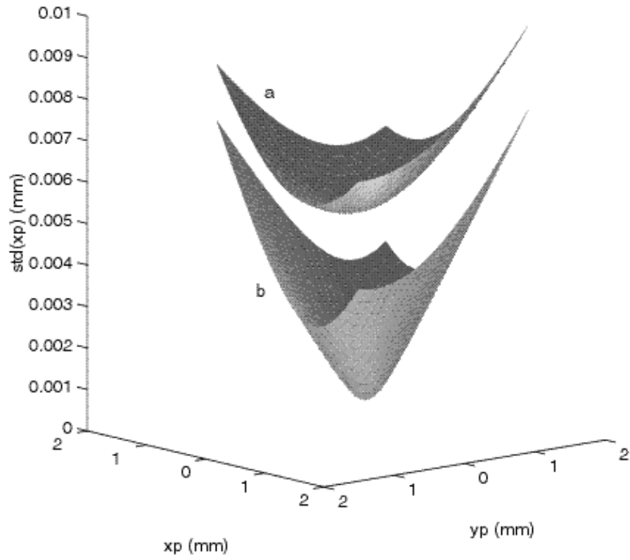
Figure 6. Effect of disturbance in image plane on topology of the objective function near the minimum point. (a) disturbance level of 6\ \mu\text{m} ; (b) disturbance level of 1\ \mu\text{m} .
