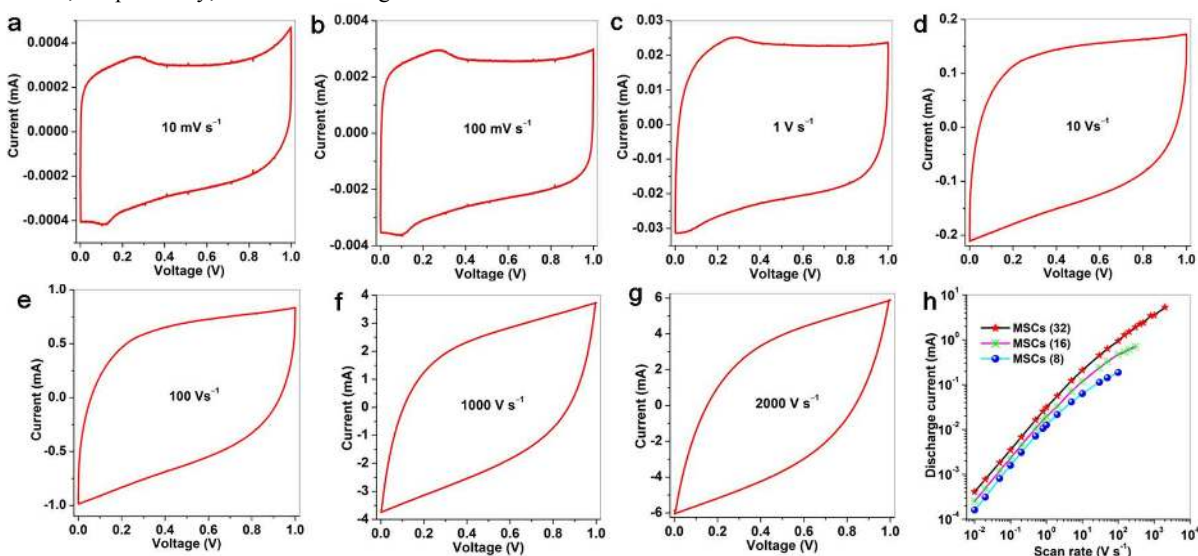
Fig. 2 (a-g) CV curves of graphene based MSCs(32) obtained at different scan rates of (a) 0.01, (b) 0.1, (c) 1, (d) 10, (e) 100, (f) 1000, and (g) 2000 \text{V s}^{-1} . (h) A plot of the discharge current as a function of scan rate for MSCs(8), MSCs(16) and MSCs(32).
