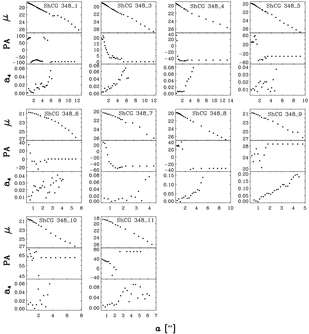
Fig. 10. The profiles a - \mu , a - PA and a - a_4 for galaxies in ShCG 348.
