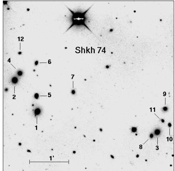
Fig. 2. The image of ShCG 74 in R . North is up, East is left.
