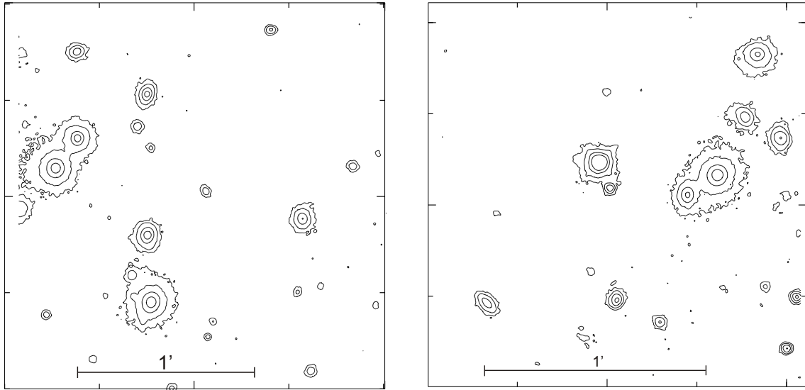
Fig. 3. The isophotal contour plots of galaxies in the eastern (left panel) and western (right panel) parts of ShCG 74.
