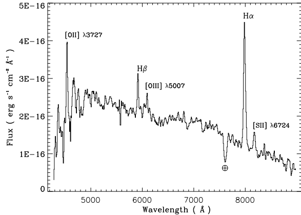
Fig. 1. The spectrum of galaxy ShCG 74-10.
