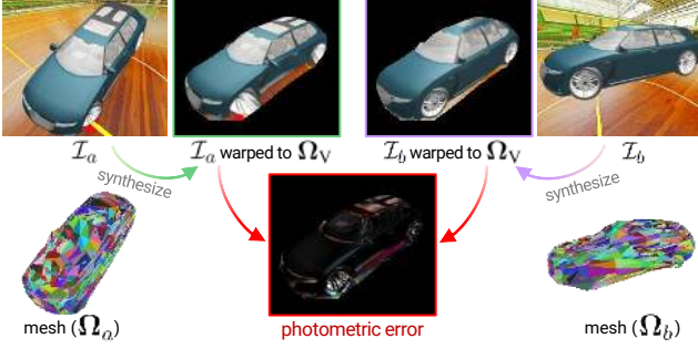
Figure 3: Visualization of the photometric loss \mathcal{L}_{\text{photo}} between the synthesized appearances at virtual viewpoints \Omega_V starting from input images \mathcal{I}_a and \mathcal{I}_b . The photometric loss \mathcal{L}_{\text{photo}} encourages consistent appearance syntheses from both input viewpoints \Omega_a and \Omega_b .
