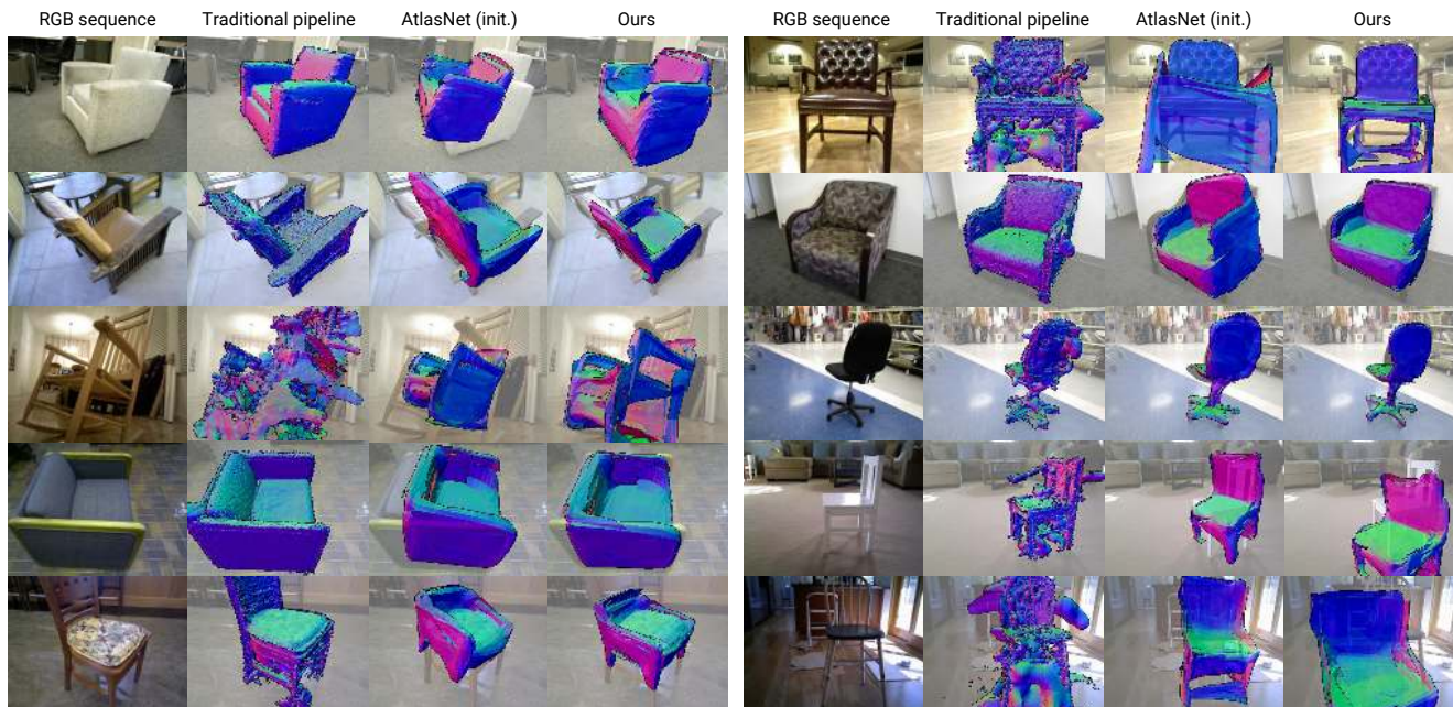
Figure 10: Qualitative results on real-world sequences. Given an initialization, our method accurately aligns a generated mesh to an RGB video. Even when the initial mesh is an inaccurate prediction of the real object, our method is still able to align the semantic parts (bottom left). We show failure cases in the last two examples in the bottom right, where there is insufficient background texture as photometric cues and where the initial mesh is insufficient to capture the thin structures. We also show the result of a traditional reconstruction pipeline [30] after manual cleanup. Due to the difficulty of the problem these meshes still often have many undesirable artifacts.
