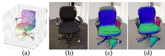
Figure 9: We select 3 correspondences between (a) the mesh vertices and (b) the SfM points to find (c) an estimated coordinate system mapping by fitting a 3D similarity transform. (d) Alignment result after our photometric optimization.
