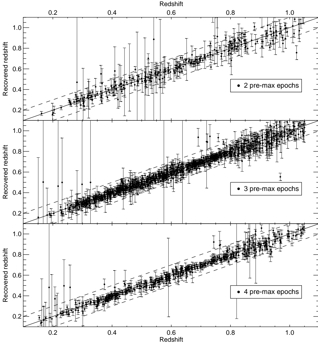
Fig. 2.— Results of the SN selection code run on a synthetic dataset of 2000 SNe Ia generated with observational parameters similar to that found in the SNLS (see § 3.2 for simulation details). This figure shows the comparison of actual and recovered redshift, and how this varies depending on the number of pre-maximum light-curve epochs are used in the fit, excluding pre-SN explosion epochs, from 2 epochs (top panel) to 4 epochs (lower panel). Only pre-maximum light data (including epochs of non detections) are used when recovering the redshift. On each epoch, 3 filters are observed, either g'r'i' or r'i'z' .
