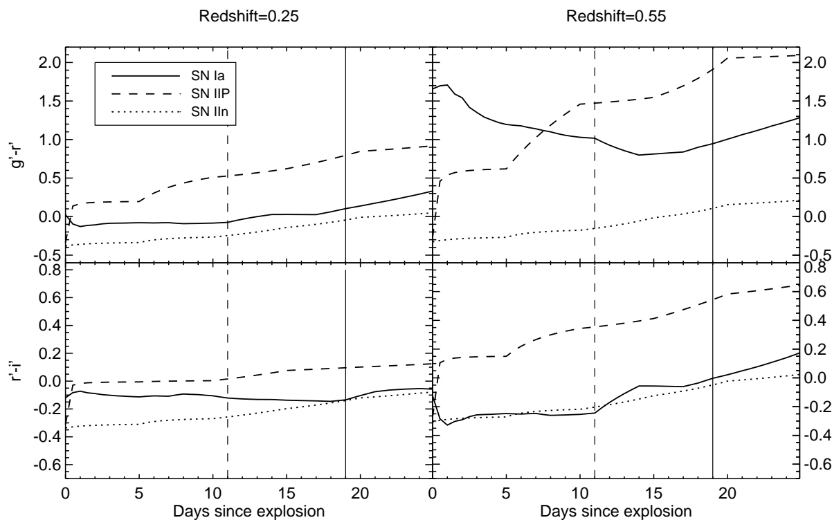
Fig. 5.— The observed g' - r' and r' - i' colors of SNe Ia compared to some SNe II models as a function of rest-frame phase of the SN. Two redshifts are shown; z = 0.25 and z = 0.55 . Note that SNe II and SNe Ia peak at different times after explosion; these are indicated with different vertical lines in the figure.
