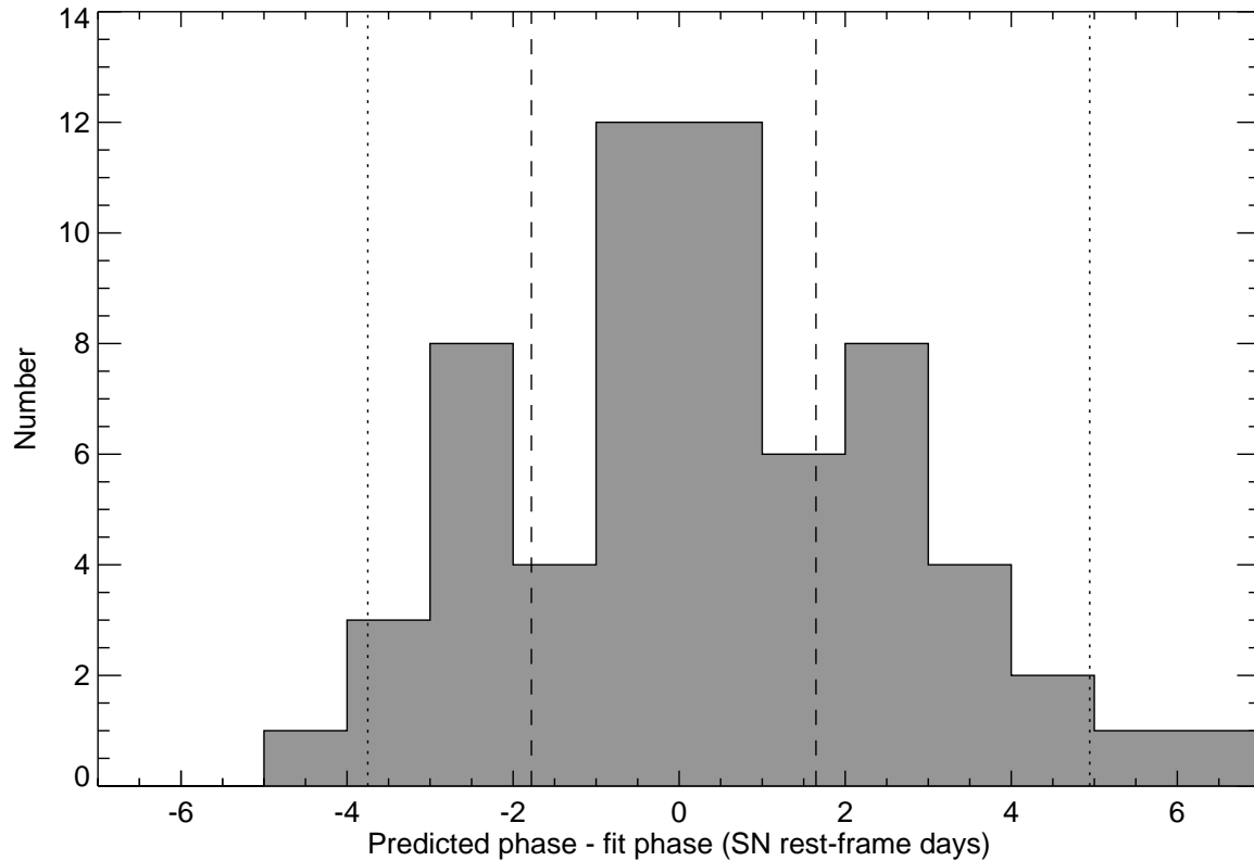
Fig. 10.— The distribution of the predicted time of maximum light minus the actual time of maximum light in the SN rest-frame. The “predicted time of maximum light” is based only on pre-maximum light light-curve data i.e. the data available at the time of spectroscopic follow-up. The “actual time of maximum light” is based on the entire SN light-curve. The vertical lines denote the region containing 50% (dashed) and 90% (dotted) of all candidates. Only confirmed SNe Ia (or SNe Ia*) with spectroscopic redshifts are shown. The uncertainty on the time of maximum light from fits based on the entire light-curve is \sim 0.5 - 1.0 days.
