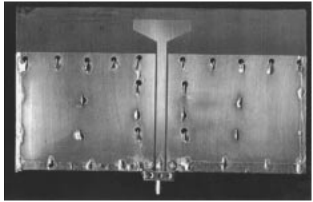
Fig. 1. Photograph of a printed tab monopole with a grounded coplanar waveguide line feed.
