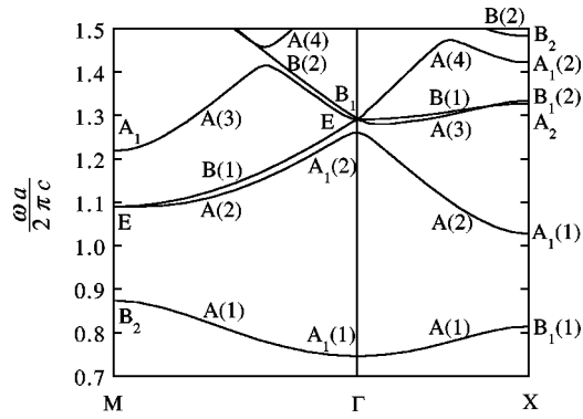
FIG. 4. The dispersion relation of the two-dimensional square photonic crystal composed of metallic cylinders (crystal 1) for the E polarization calculated by means of the numerical simulation of the dipole radiation. The ordinate is the normalized frequency where \omega , a , and c stand for the angular frequency of the radiation field, the lattice constant of the crystal, and the light velocity in free space. According to the previous calculation by Kuzmiak et al. (Refs. 6–8), the following parameters were used for numerical calculation: r_m/a=0.472 ( f=0.7 ), where r_m denotes the radius of the metallic cylinders, \epsilon_\infty=1.0 , \omega_p a/2\pi c=1.0 , and \gamma=0.01\omega_p in Eq. (7). The dispersion relation was drawn for highly symmetric points in the first Brillouin zone of the two-dimensional crystal: \Gamma(0,0) , X(\pi/a,0) , and M(\pi/a,\pi/a) . The spatial symmetry of each eigenmode for E_z is also shown in this figure, where the number in parentheses is given in order of the ascending frequency when there is more than one mode of the same symmetry in the analyzed frequency region.
