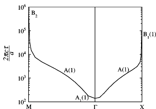
FIG. 10. The lifetime of the lowest eigenmode of crystal 2. The same parameters as for Fig. 9 were used for numerical calculation. The ordinate denotes the normalized lifetime in a logarithmic scale.
