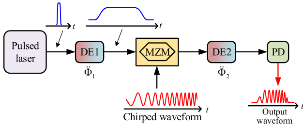
FIGURE 15. Frequency and bandwidth multiplication based on photonic time compression with a dispersion configuration of \text{sgn}(\dot{\Phi}_2) = -\text{sgn}(\dot{\Phi}_1) and |\dot{\Phi}_2| < |\dot{\Phi}_1| (DE: dispersive element; MZM: Mach-Zehnder modulator; PD: photodetector).
