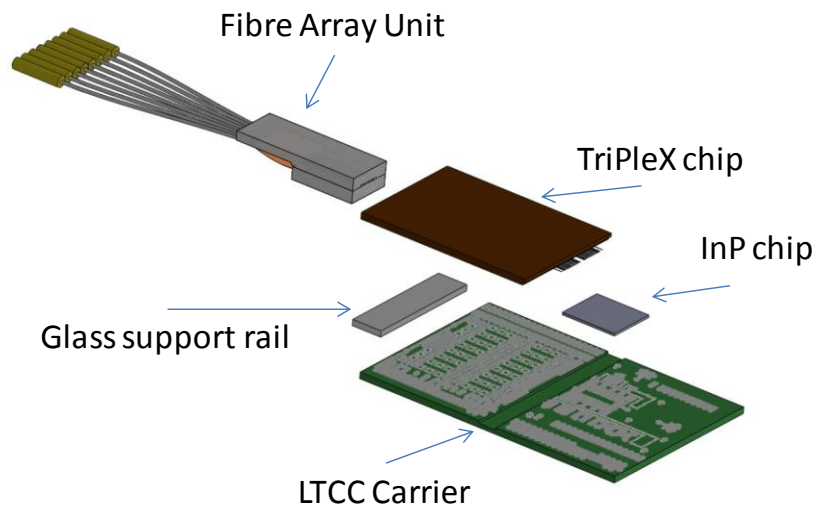
Figure 1. Exploded drawing of assembly showing the piece parts required - Fiber array unit (FAU), TriPleX chip (backside view), glass rail for mechanical FAU support, InP chip (backside view), LTCC carrier (top view).
