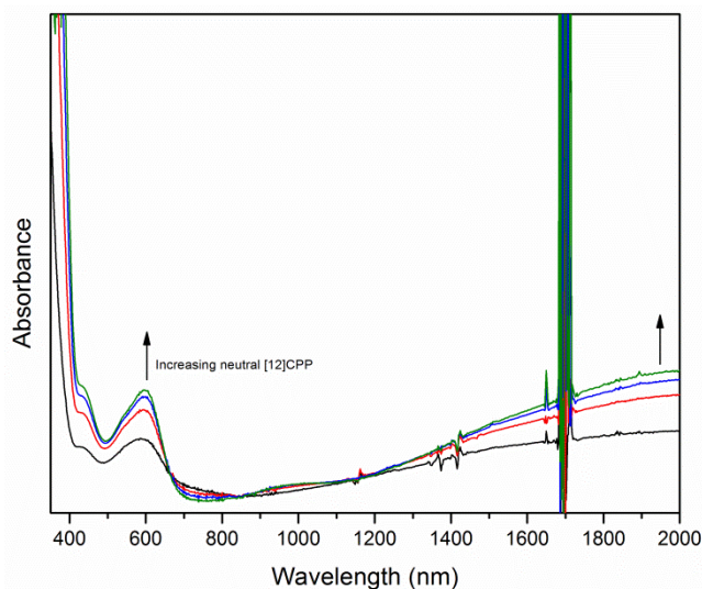
Figure S11. UV-vis-NIR spectra after the oxidation of [12]CPP (with increasing concentrations of neutral [12]CPP added)
