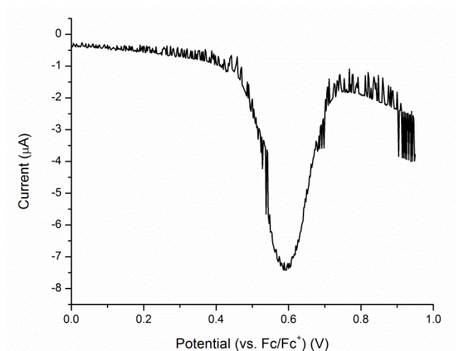
Figure S6. Differential pulse voltammogram of radical cation 1 + (0.1 M n\text{-Bu}_4\text{PF}_6 in \text{CH}_2\text{Cl}_2 ) (pulse height = 25 mV, scan increment = 2 mV)
