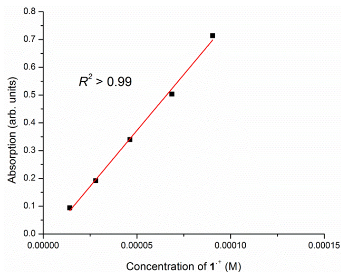
Figure S2. Beer-Lambert plot of 1^{+} at 535 nm ( \epsilon = 0.81 (\pm 0.03) \times 10^4 \text{ M}^{-1} \text{ cm}^{-1} )
