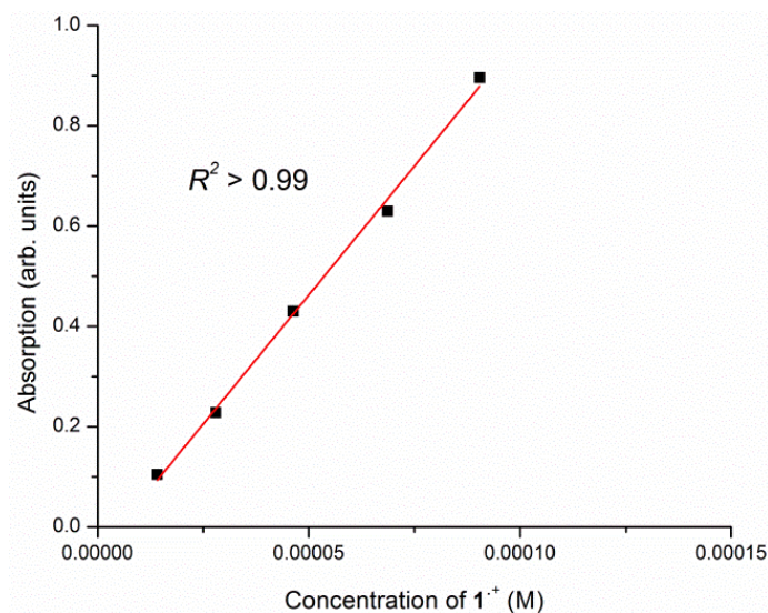
Figure S3. Beer-Lambert plot of 1^+ at 1115 nm ( \epsilon = 1.03 (\pm 0.03) \times 10^4 \text{ M}^{-1} \text{ cm}^{-1} ).
