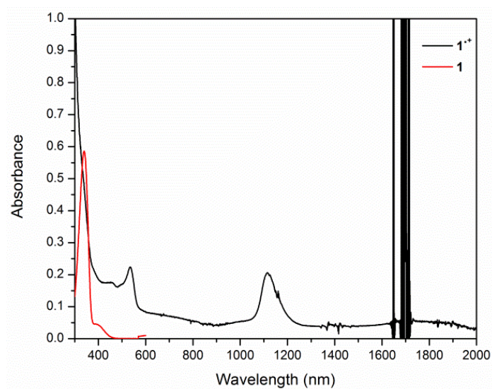
Figure S1. UV-vis-NIR spectrum of 1^{+} ( 2.7 \times 10^{-4} M) and 1 ( 6.4 \times 10^{-6} M). The absence of an absorption at 340 nm and a CR band in the NIR confirms the purity of 1^{+} .
