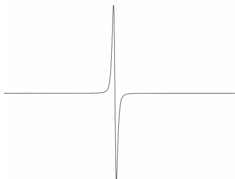
Figure S9. X-band EPR spectrum of charge-resonance dimer (\mathbf{1})_2^{+\cdot} in \text{CH}_2\text{Cl}_2 after the completion of titration experiments (Frequency = 9.389929 GHz, g = 2.007 G)
