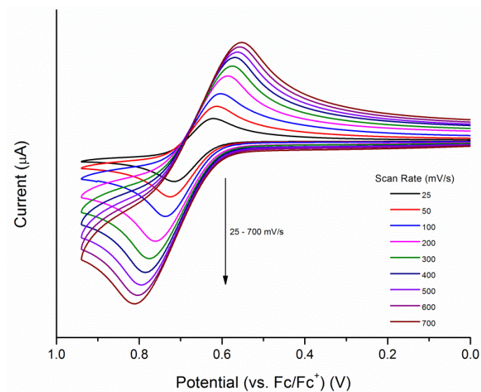
Figure S4. Cyclic voltammograms of 1 ( 1 \times 10^{-3} \text{ M} ) at increasing scan rates (25 mV/s \rightarrow 700 mV/s) (0.1 M n -Bu _4 PF _6 in CH _2 Cl _2 )
