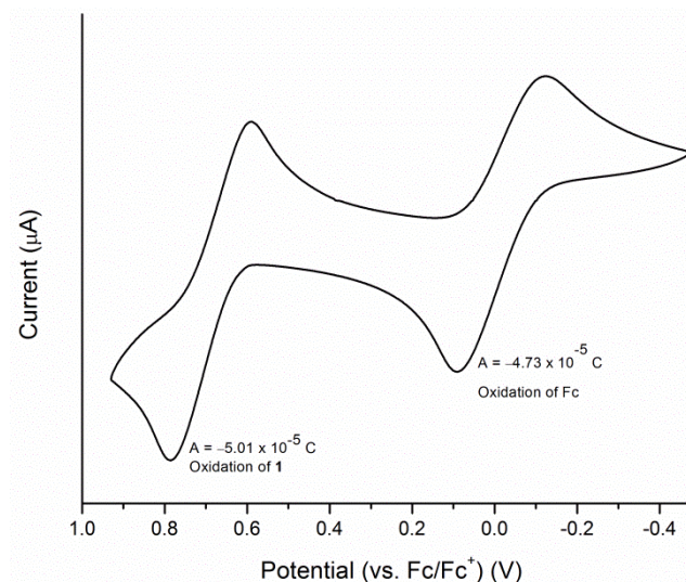
Figure S5. Cyclic voltammogram of 1 ( 1 \times 10^{-3} M) containing 1 equivalent of ferrocene (0.1 M n\text{-Bu}_4\text{PF}_6 in \text{CH}_2\text{Cl}_2 , scan rate = 50 mV/s). A_1 / A_{\text{Fc}} = 1.06 .
