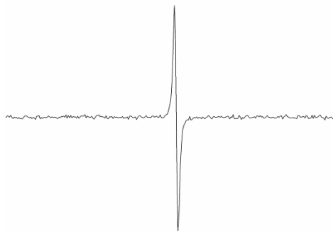
Figure S12. X-band EPR spectrum of ([12]\text{CPP})_2^{\cdot+} after optical titration experiments ( \text{CH}_2\text{Cl}_2 ) (Frequency = 9.857404 GHz, g = 2.006 )
