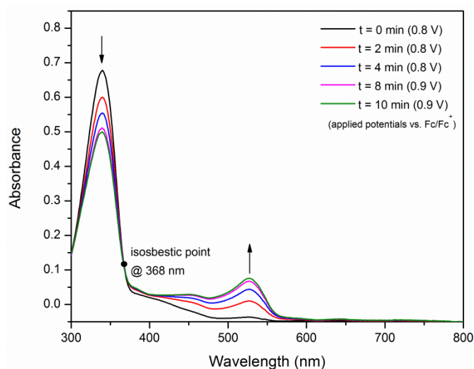
Figure S7. UV-vis spectrum (in CH 2 Cl 2 ) depicting the gradual oxidation over time of neutral 1 to radical cation 1 •+ with an applied potential. Applied potentials are all relative to the Fc/Fc + couple for consistency when referring to cyclic voltammogram (Figure S4)
